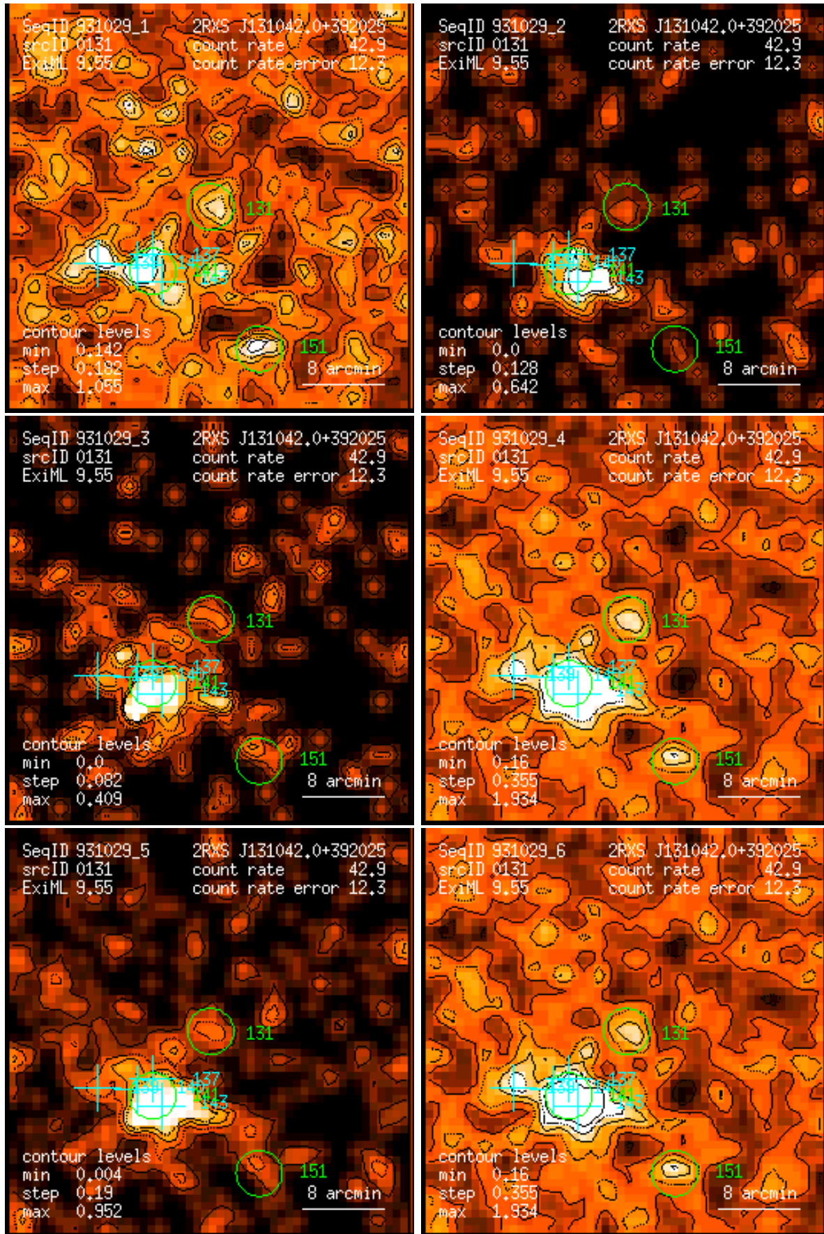
Figure 131: RASS 931029: detection 0131: band rate images, Gaussian filter: (1) PSPC channels 11 – 41, (2) 52 – 90, (3) 91 – 201, (4) 11 – 235, (5) 52 – 201, (6) 11 – 201. Broad band rates in counts/ks. Band rate contour levels in counts/ks/arcmin 2 .
