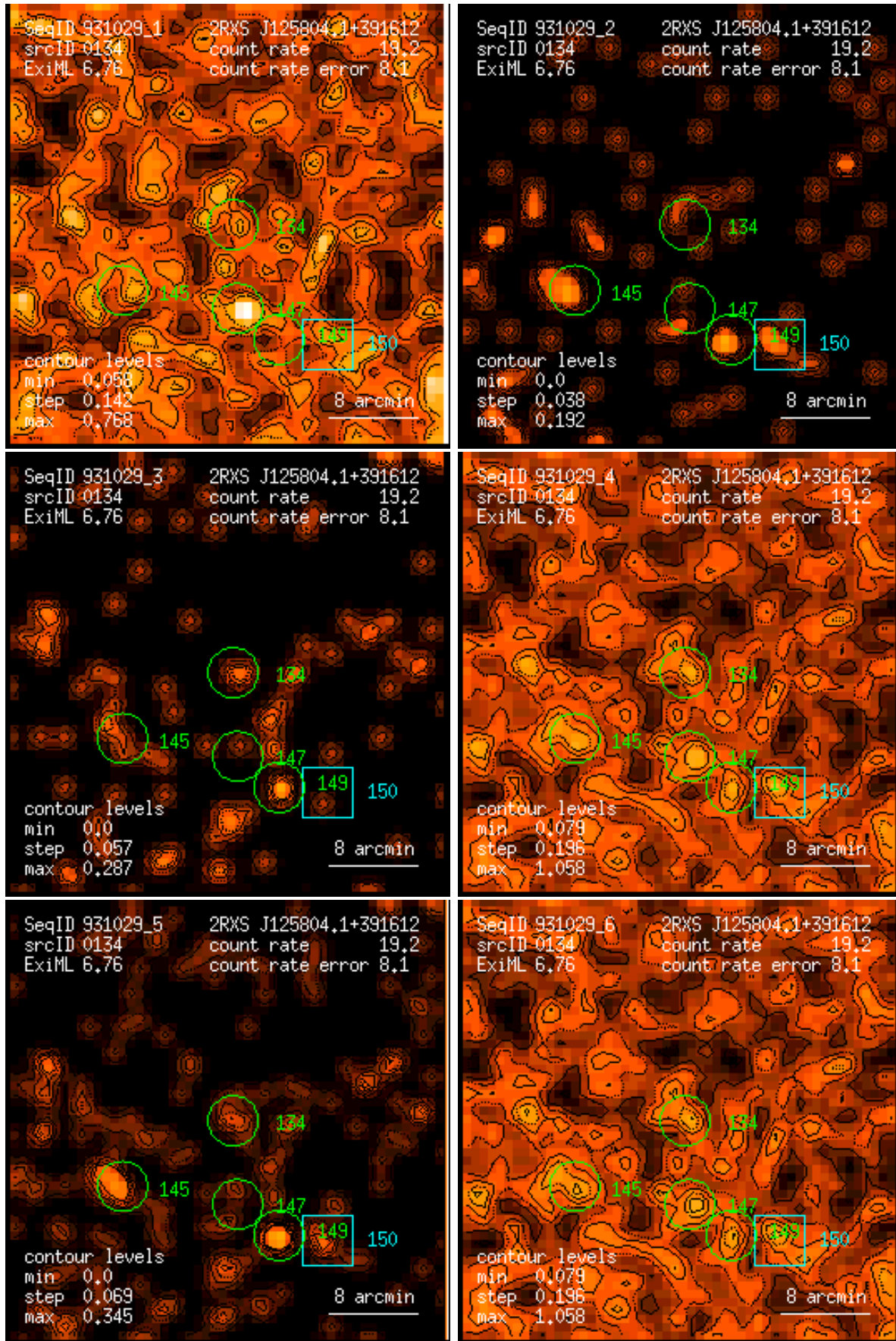
Figure 134: RASS 931029: detection 0134: band rate images, Gaussian filter: (1) PSPC channels 11 – 41, (2) 52 – 90, (3) 91 – 201, (4) 11 – 235, (5) 52 – 201, (6) 11 – 201. Broad band rates in counts/ks. Band rate contour levels in counts/ks/arcmin 2 .
