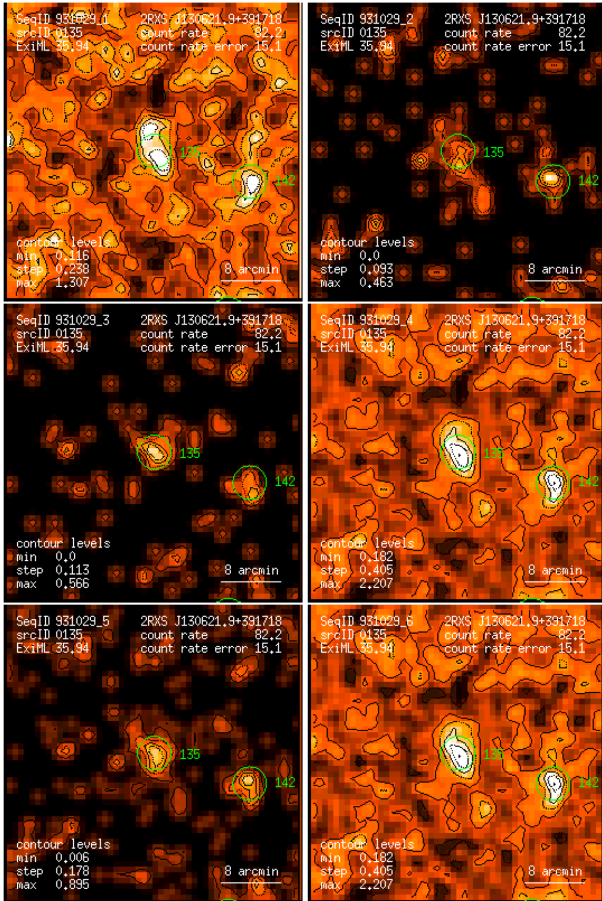
Figure 135: RASS 931029: detection 0135: band rate images, Gaussian filter: (1) PSPC channels 11 – 41, (2) 52 – 90, (3) 91 – 201, (4) 11 – 235, (5) 52 – 201, (6) 11 – 201. Broad band rates in counts/ks. Band rate contour levels in counts/ks/arcmin 2 .
