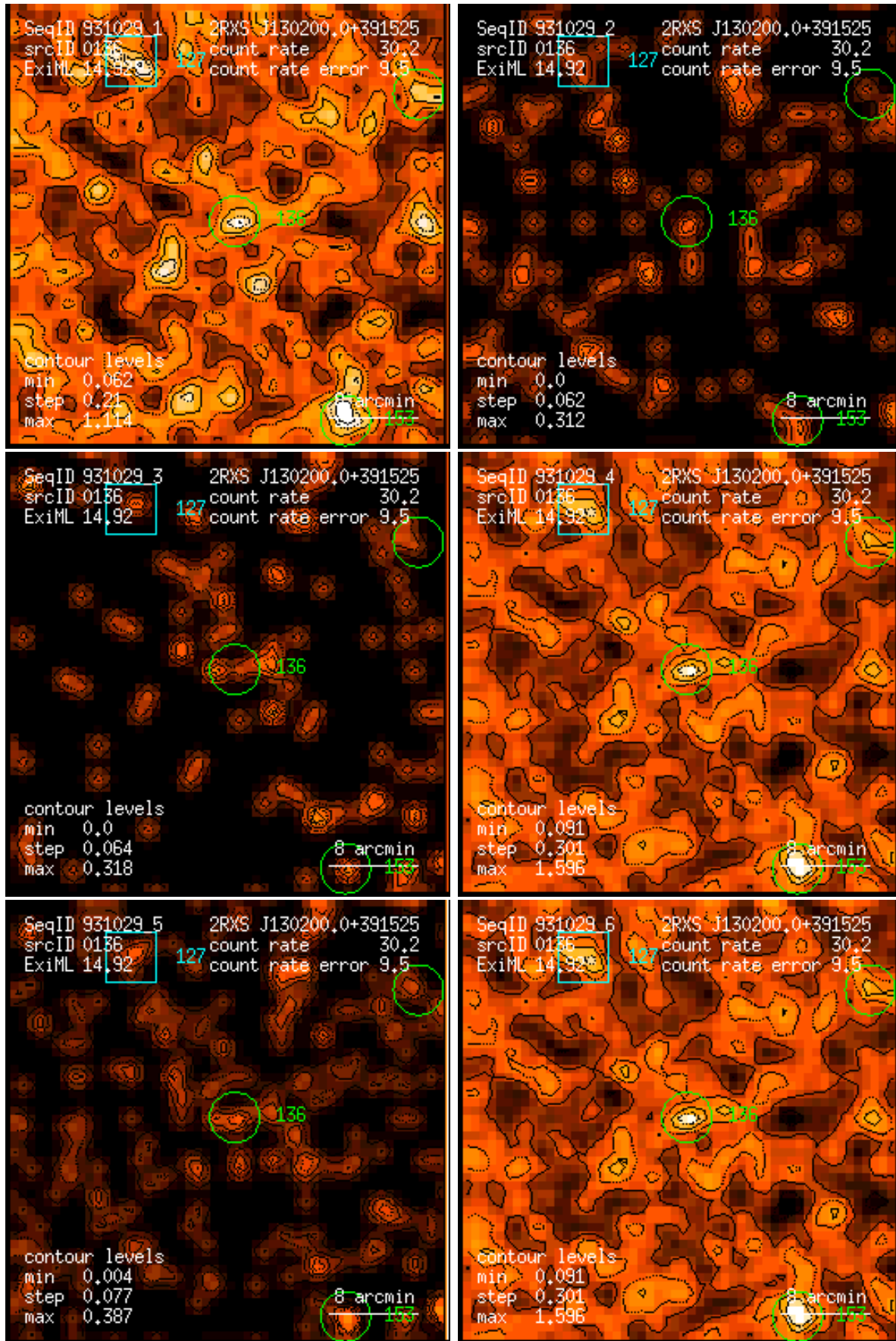
Figure 136: RASS 931029: detection 0136: band rate images, Gaussian filter: (1) PSPC channels 11 – 41, (2) 52 – 90, (3) 91 – 201, (4) 11 – 235, (5) 52 – 201, (6) 11 – 201. Broad band rates in counts/ks. Band rate contour levels in counts/ks/arcmin 2 .
