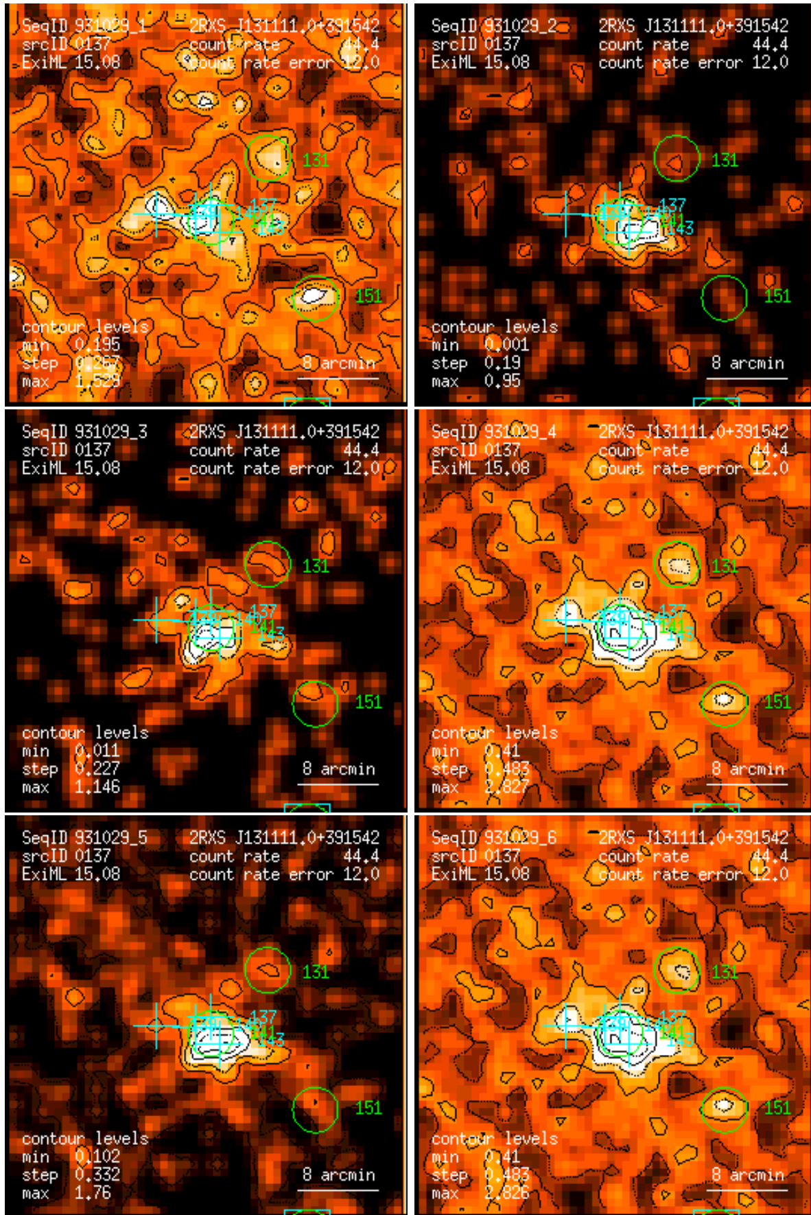
Figure 137: RASS 931029: detection 0137: band rate images, Gaussian filter: (1) PSPC channels 11 – 41, (2) 52 – 90, (3) 91 – 201, (4) 11 – 235, (5) 52 – 201, (6) 11 – 201. Broad band rates in counts/ks. Band rate contour levels in counts/ks/arcmin 2 .
