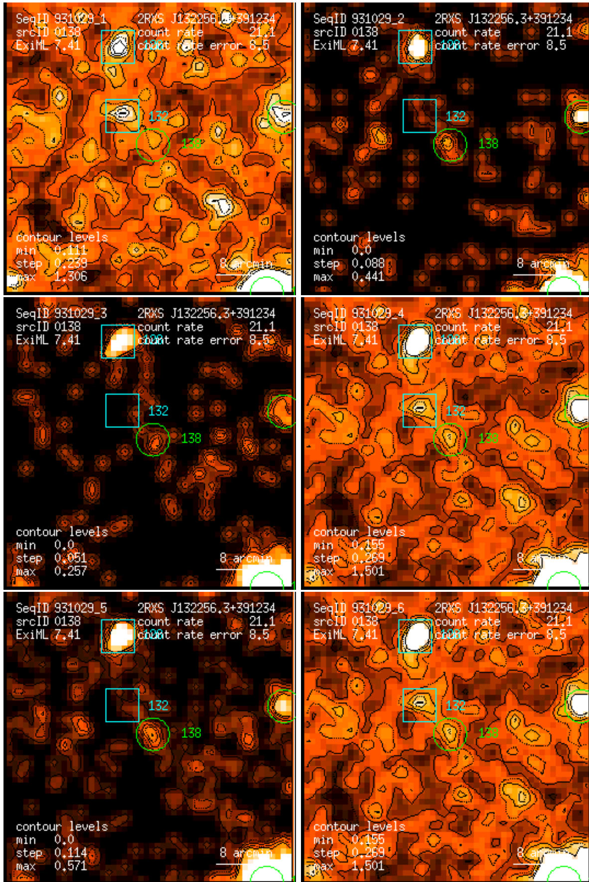
Figure 138: RASS 931029: detection 0138: band rate images, Gaussian filter: (1) PSPC channels 11 – 41, (2) 52 – 90, (3) 91 – 201, (4) 11 – 235, (5) 52 – 201, (6) 11 – 201. Broad band rates in counts/ks. Band rate contour levels in counts/ks/arcmin 2 .
