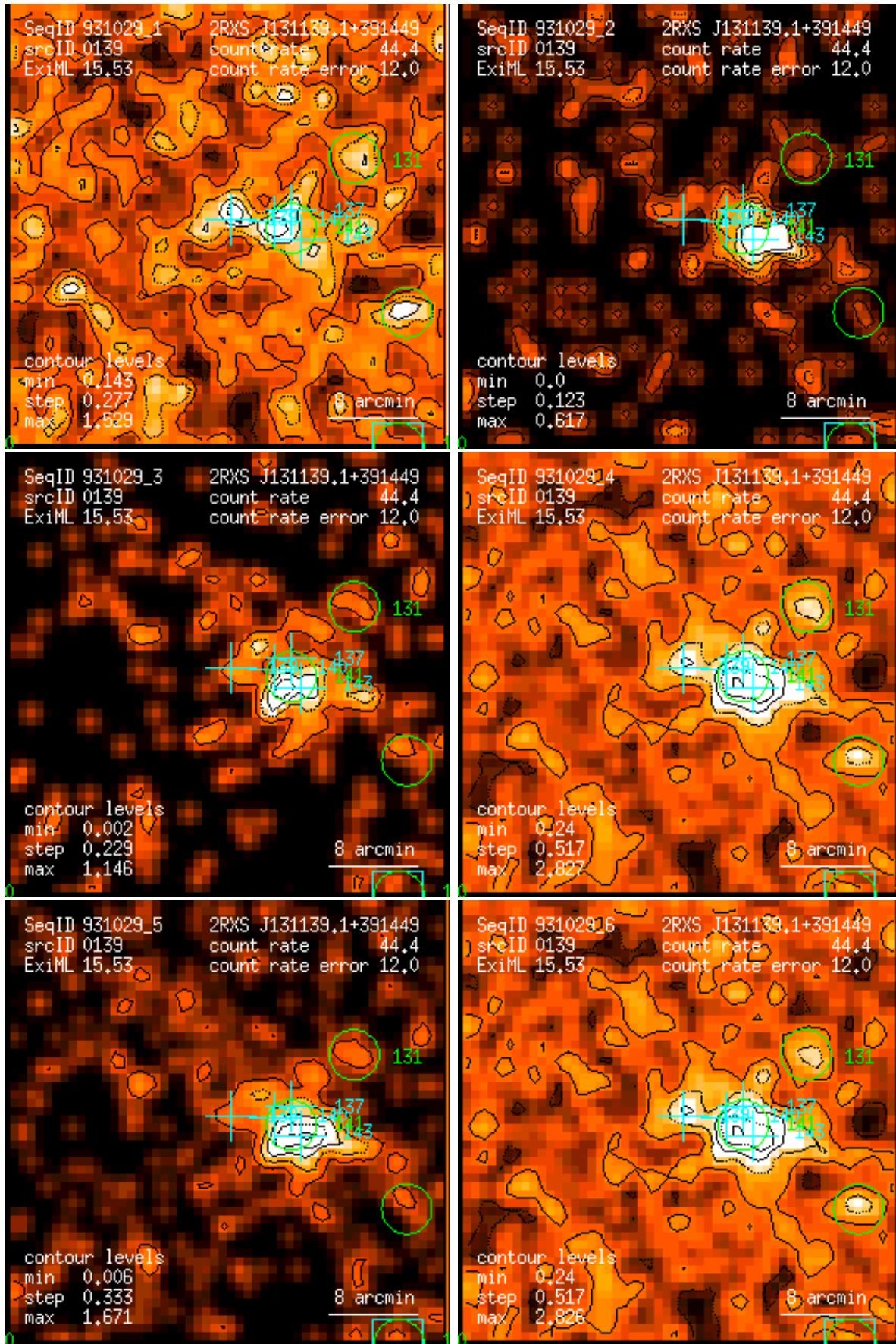
Figure 139: RASS 931029: detection 0139: band rate images, Gaussian filter: (1) PSPC channels 11 – 41, (2) 52 – 90, (3) 91 – 201, (4) 11 – 235, (5) 52 – 201, (6) 11 – 201. Broad band rates in counts/ks. Band rate contour levels in counts/ks/arcmin 2 .
