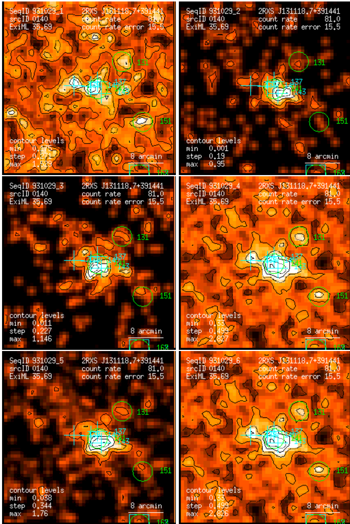
Figure 140: RASS 931029: detection 0140: band rate images, Gaussian filter: (1) PSPC channels 11 – 41, (2) 52 – 90, (3) 91 – 201, (4) 11 – 235, (5) 52 – 201, (6) 11 – 201. Broad band rates in counts/ks. Band rate contour levels in counts/ks/arcmin 2 .
