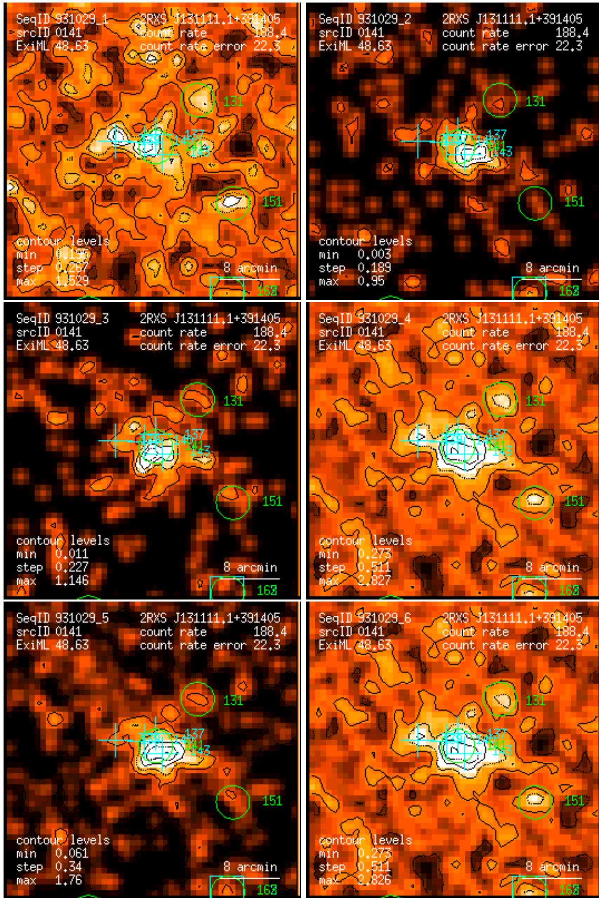
Figure 141: RASS 931029: detection 0141: band rate images, Gaussian filter: (1) PSPC channels 11 – 41, (2) 52 – 90, (3) 91 – 201, (4) 11 – 235, (5) 52 – 201, (6) 11 – 201. Broad band rates in counts/ks. Band rate contour levels in counts/ks/arcmin 2 .
