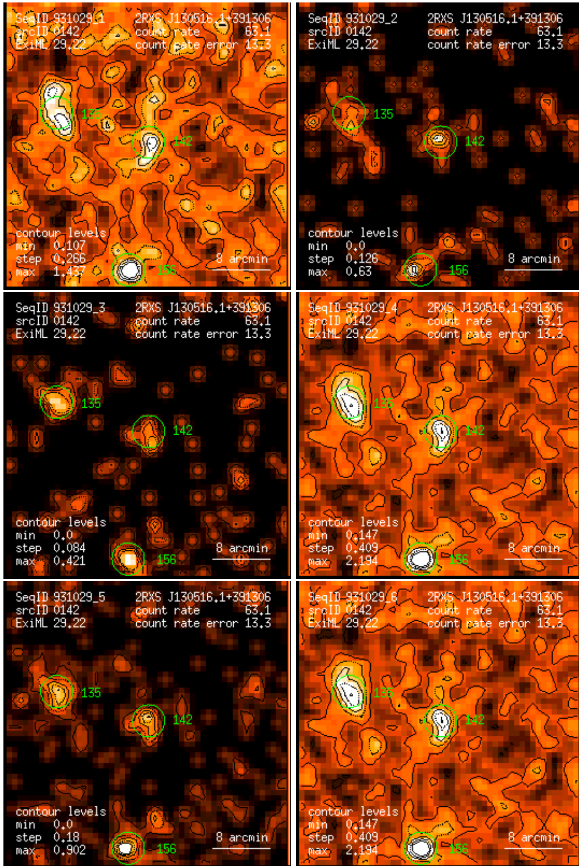
Figure 142: RASS 931029: detection 0142: band rate images, Gaussian filter: (1) PSPC channels 11 – 41, (2) 52 – 90, (3) 91 – 201, (4) 11 – 235, (5) 52 – 201, (6) 11 – 201. Broad band rates in counts/ks. Band rate contour levels in counts/ks/arcmin 2 .
