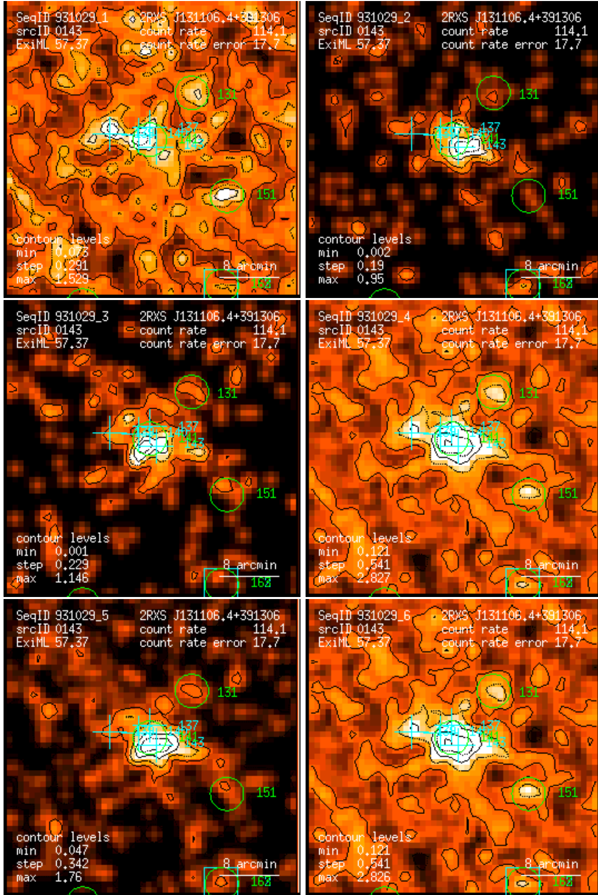
Figure 143: RASS 931029: detection 0143: band rate images, Gaussian filter: (1) PSPC channels 11 – 41, (2) 52 – 90, (3) 91 – 201, (4) 11 – 235, (5) 52 – 201, (6) 11 – 201. Broad band rates in counts/ks. Band rate contour levels in counts/ks/arcmin 2 .
