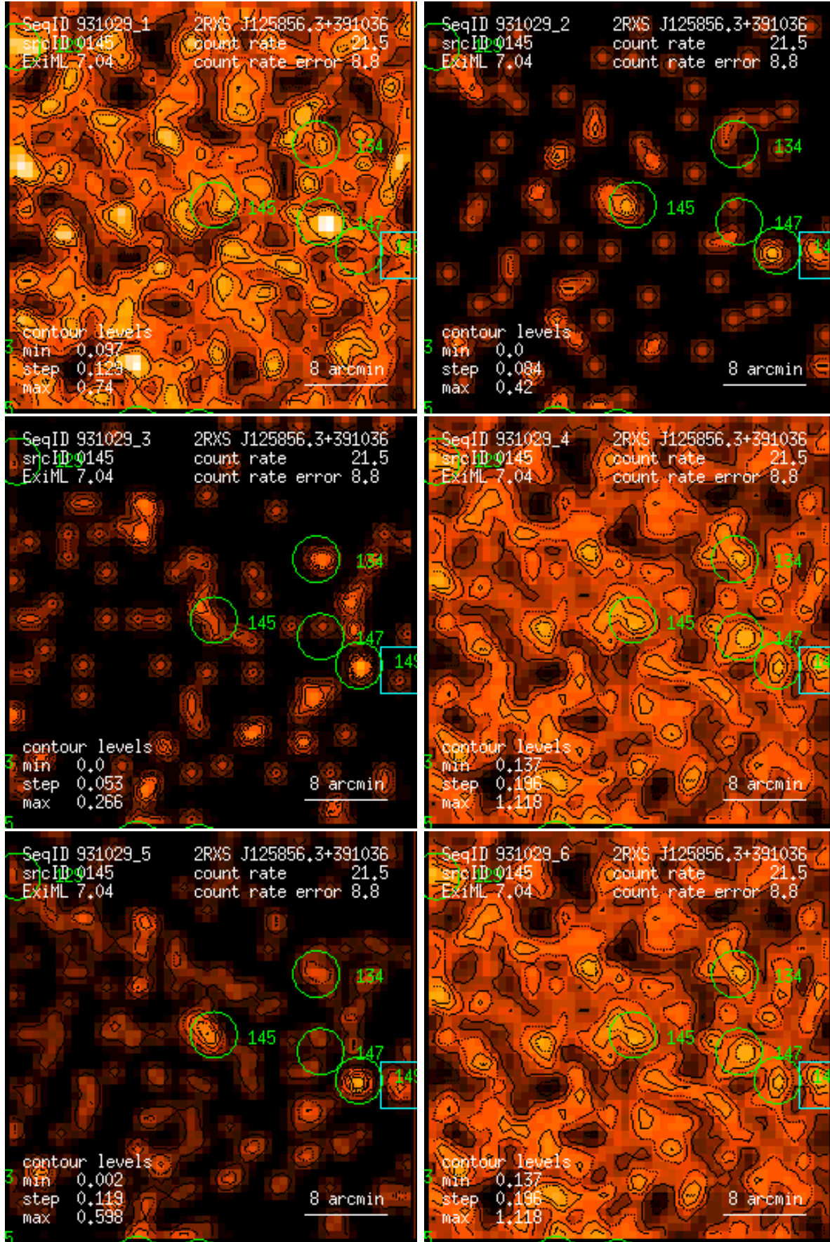
Figure 145: RASS 931029: detection 0145: band rate images, Gaussian filter: (1) PSPC channels 11 – 41, (2) 52 – 90, (3) 91 – 201, (4) 11 – 235, (5) 52 – 201, (6) 11 – 201. Broad band rates in counts/ks. Band rate contour levels in counts/ks/arcmin 2 .
