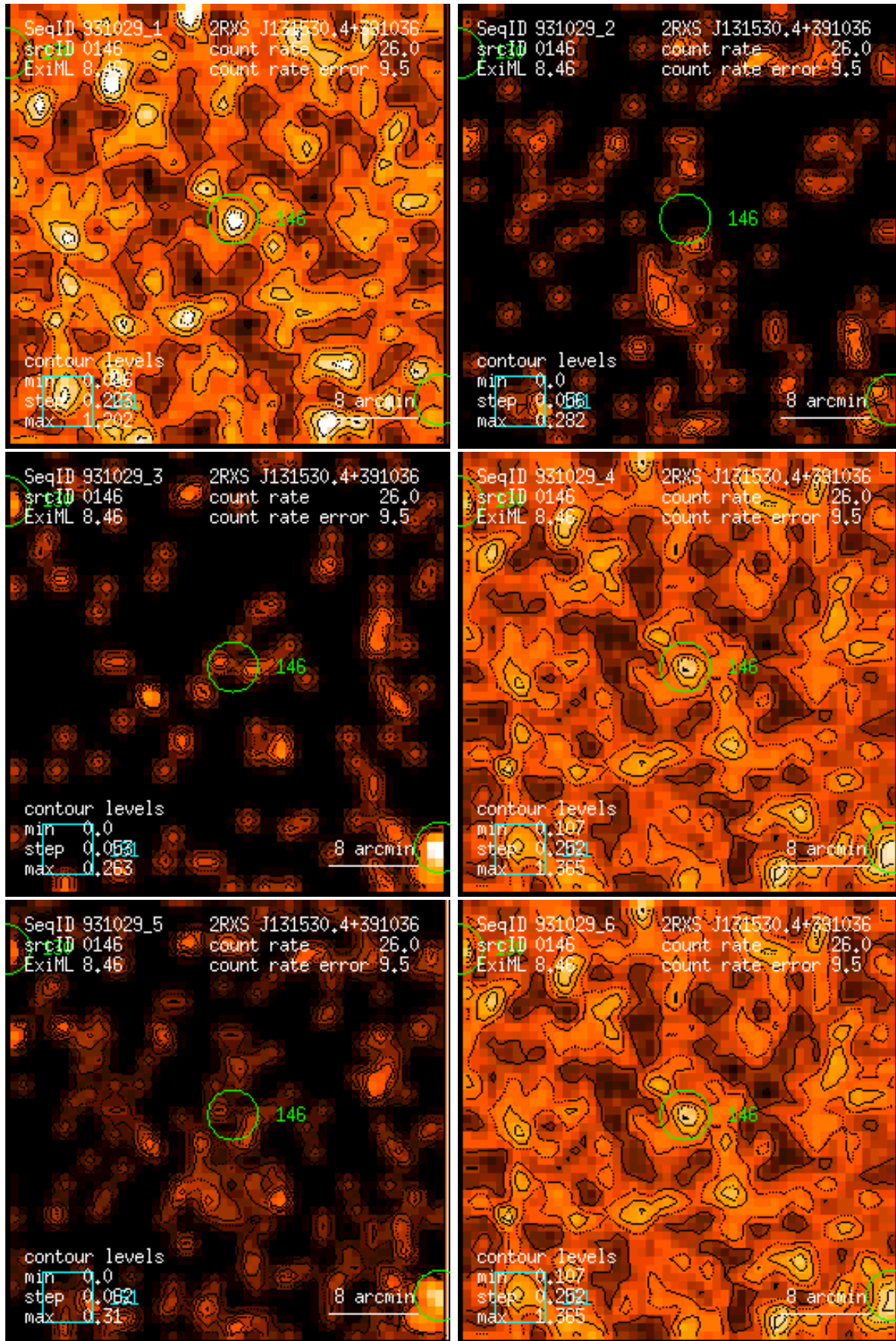
Figure 146: RASS 931029: detection 0146: band rate images, Gaussian filter: (1) PSPC channels 11 – 41, (2) 52 – 90, (3) 91 – 201, (4) 11 – 235, (5) 52 – 201, (6) 11 – 201. Broad band rates in counts/ks. Band rate contour levels in counts/ks/arcmin 2 .
