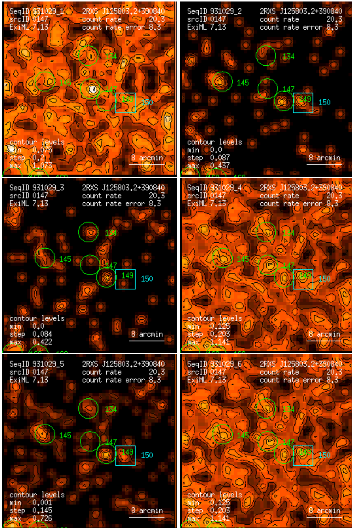
Figure 147: RASS 931029: detection 0147: band rate images, Gaussian filter: (1) PSPC channels 11 – 41, (2) 52 – 90, (3) 91 – 201, (4) 11 – 235, (5) 52 – 201, (6) 11 – 201. Broad band rates in counts/ks. Band rate contour levels in counts/ks/arcmin 2 .
