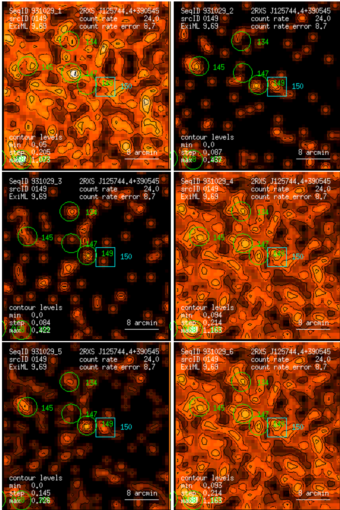
Figure 149: RASS 931029: detection 0149: band rate images, Gaussian filter: (1) PSPC channels 11 – 41, (2) 52 – 90, (3) 91 – 201, (4) 11 – 235, (5) 52 – 201, (6) 11 – 201. Broad band rates in counts/ks. Band rate contour levels in counts/ks/arcmin 2 .
