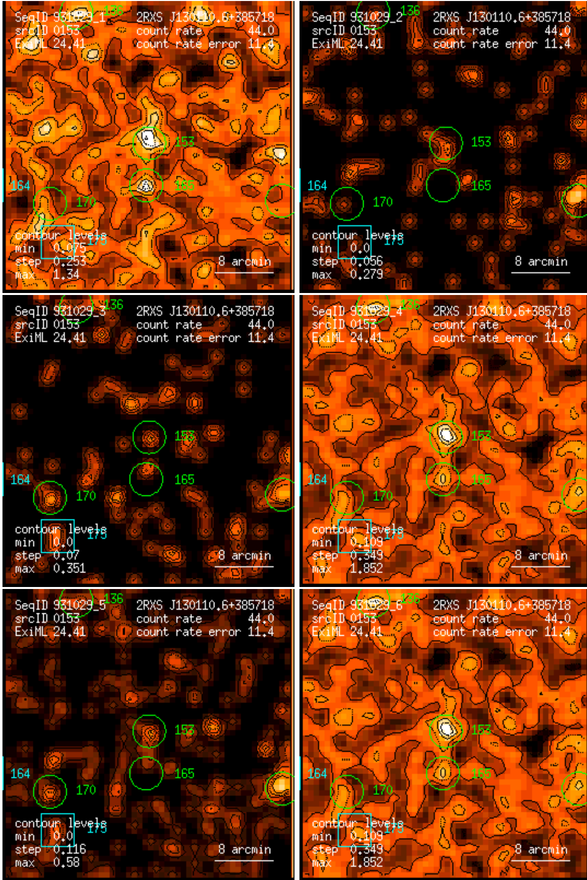
Figure 153: RASS 931029: detection 0153: band rate images, Gaussian filter: (1) PSPC channels 11 – 41, (2) 52 – 90, (3) 91 – 201, (4) 11 – 235, (5) 52 – 201, (6) 11 – 201. Broad band rates in counts/ks. Band rate contour levels in counts/ks/arcmin 2 .
