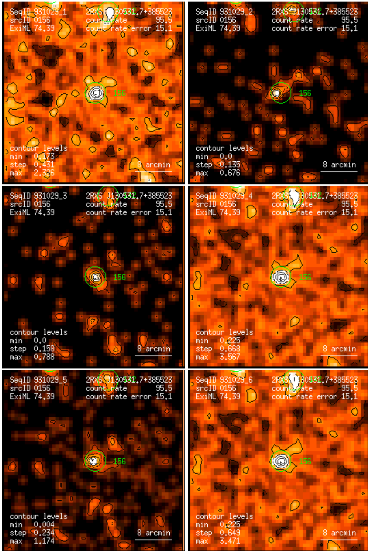
Figure 156: RASS 931029: detection 0156: band rate images, Gaussian filter: (1) PSPC channels 11 – 41, (2) 52 – 90, (3) 91 – 201, (4) 11 – 235, (5) 52 – 201, (6) 11 – 201. Broad band rates in counts/ks. Band rate contour levels in counts/ks/arcmin 2 .
