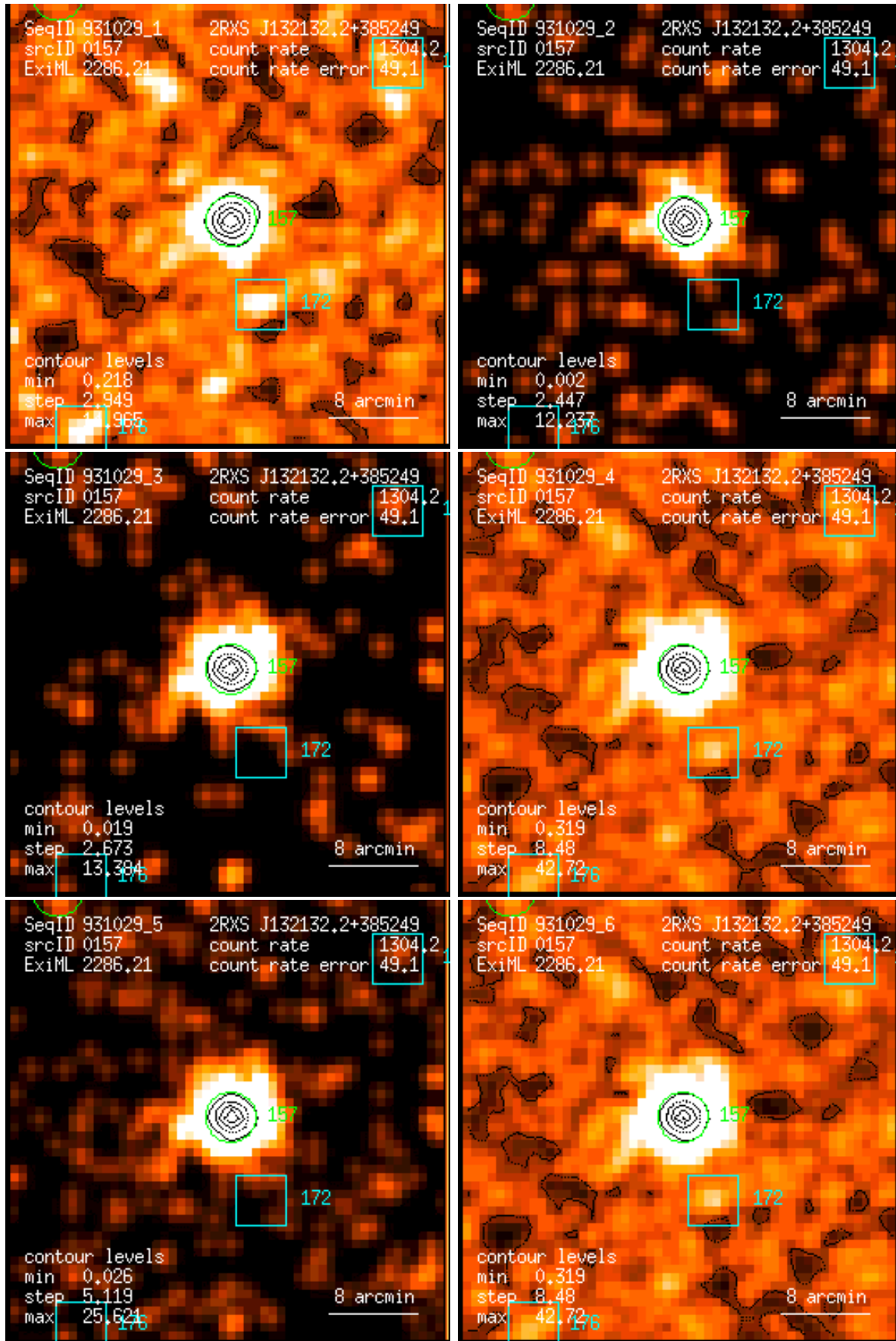
Figure 157: RASS 931029: detection 0157: band rate images, Gaussian filter: (1) PSPC channels 11 – 41, (2) 52 – 90, (3) 91 – 201, (4) 11 – 235, (5) 52 – 201, (6) 11 – 201. Broad band rates in counts/ks. Band rate contour levels in counts/ks/arcmin 2 .
