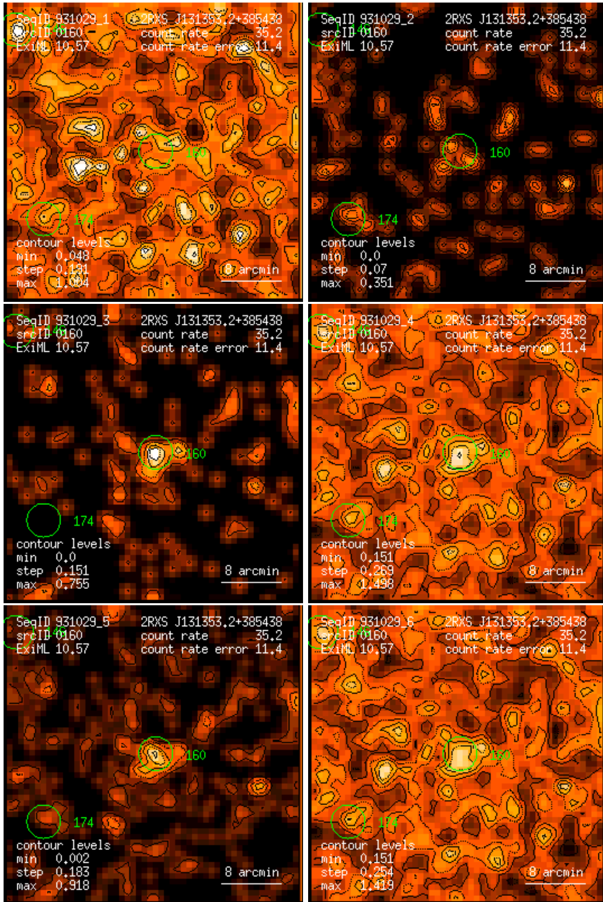
Figure 160: RASS 931029: detection 0160: band rate images, Gaussian filter: (1) PSPC channels 11 – 41, (2) 52 – 90, (3) 91 – 201, (4) 11 – 235, (5) 52 – 201, (6) 11 – 201. Broad band rates in counts/ks. Band rate contour levels in counts/ks/arcmin 2 .
