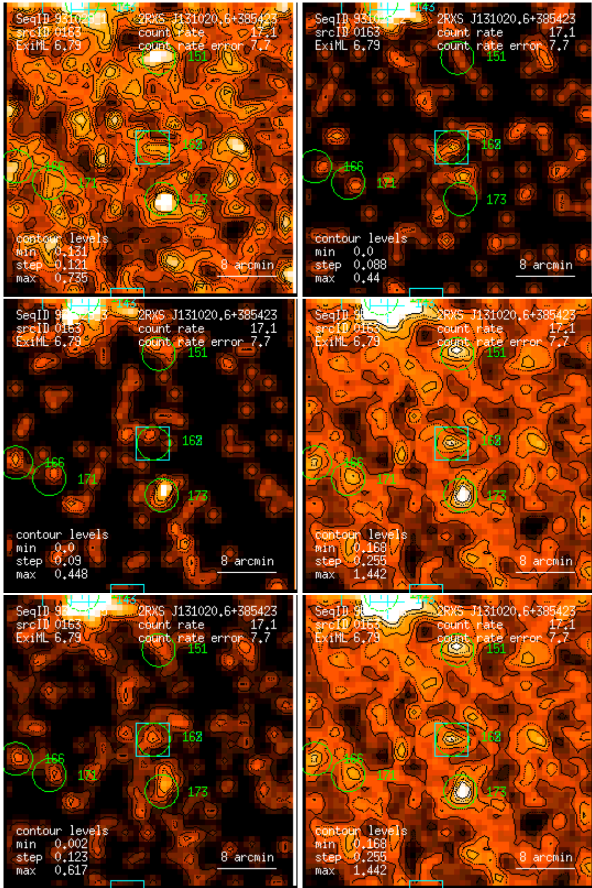
Figure 163: RASS 931029: detection 0163: band rate images, Gaussian filter: (1) PSPC channels 11 – 41, (2) 52 – 90, (3) 91 – 201, (4) 11 – 235, (5) 52 – 201, (6) 11 – 201. Broad band rates in counts/ks. Band rate contour levels in counts/ks/arcmin 2 .
