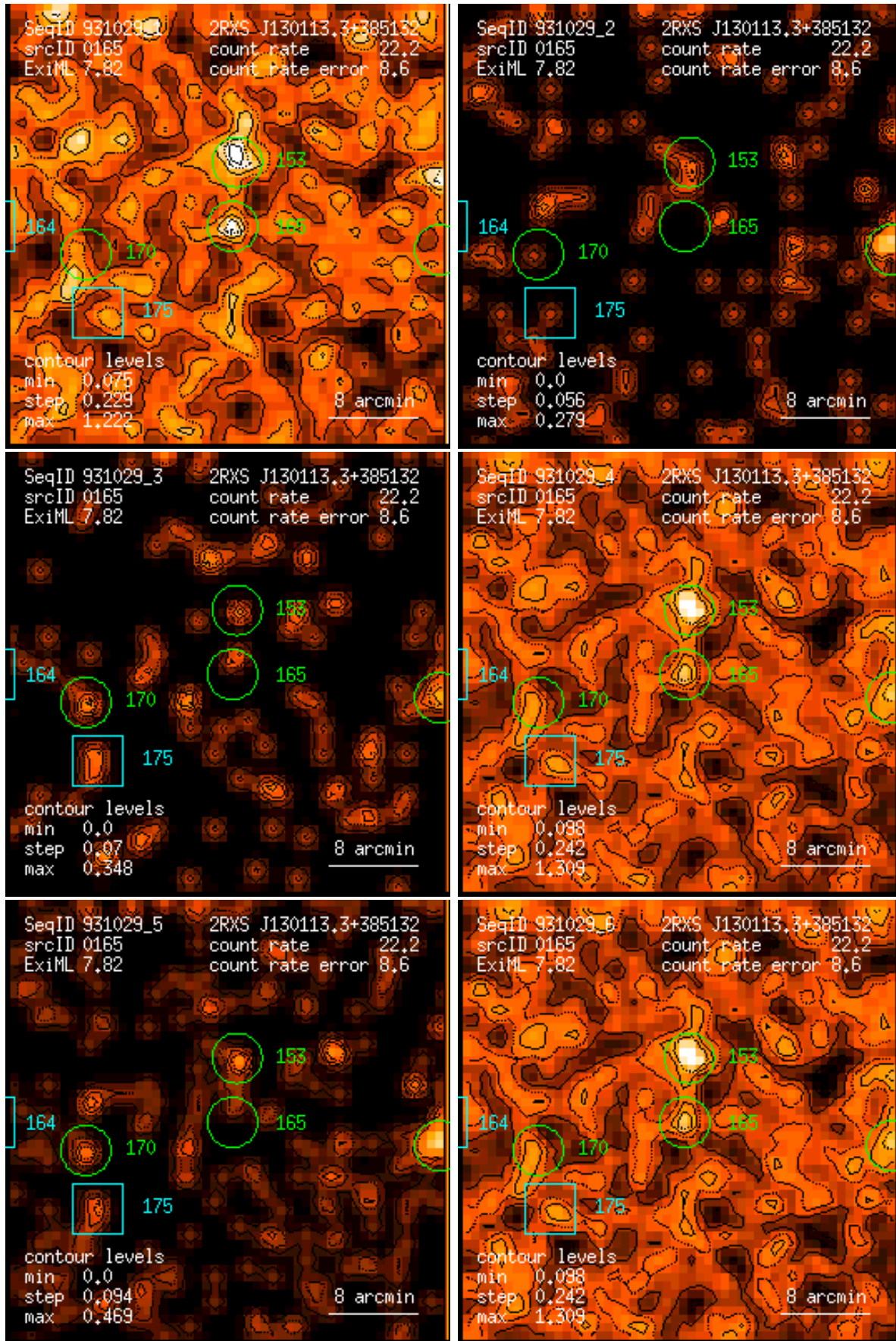
Figure 165: RASS 931029: detection 0165: band rate images, Gaussian filter: (1) PSPC channels 11 – 41, (2) 52 – 90, (3) 91 – 201, (4) 11 – 235, (5) 52 – 201, (6) 11 – 201. Broad band rates in counts/ks. Band rate contour levels in counts/ks/arcmin 2 .
