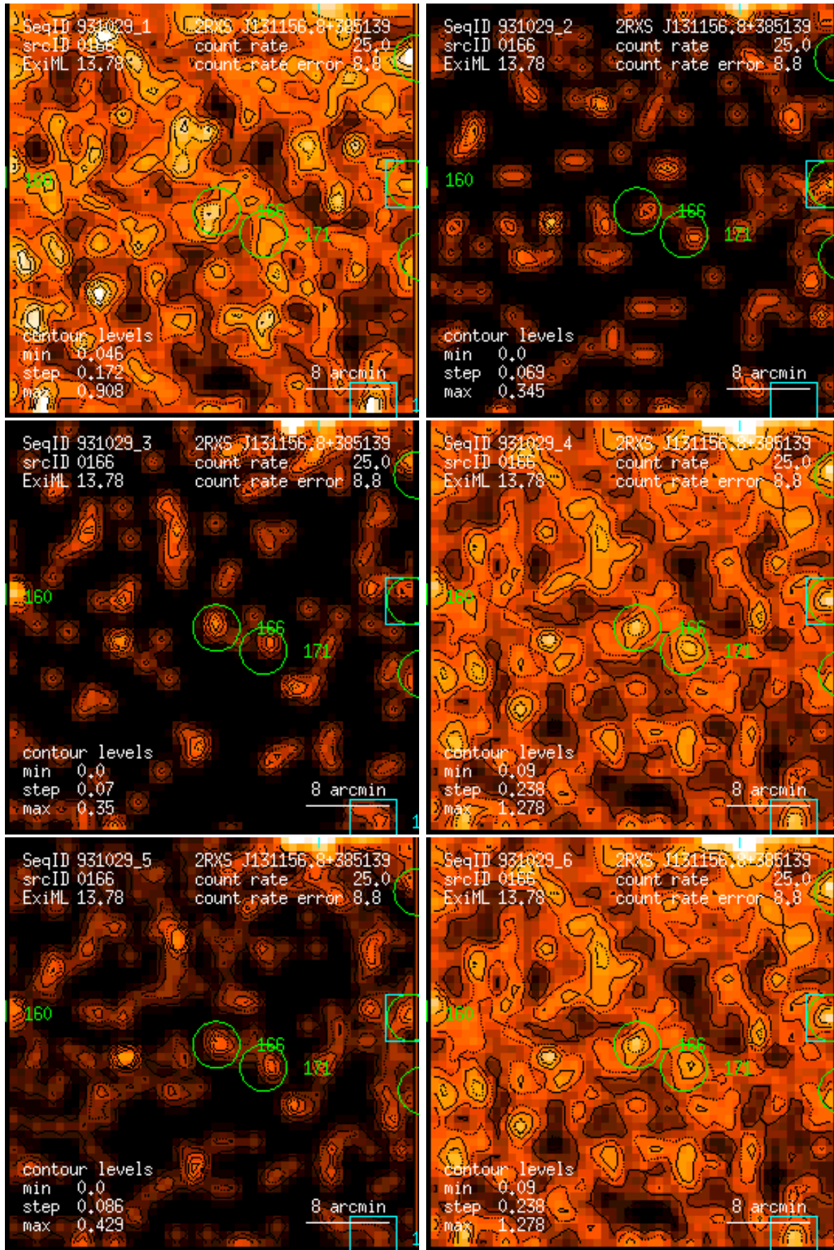
Figure 166: RASS 931029: detection 0166: band rate images, Gaussian filter: (1) PSPC channels 11 – 41, (2) 52 – 90, (3) 91 – 201, (4) 11 – 235, (5) 52 – 201, (6) 11 – 201. Broad band rates in counts/ks. Band rate contour levels in counts/ks/arcmin 2 .
