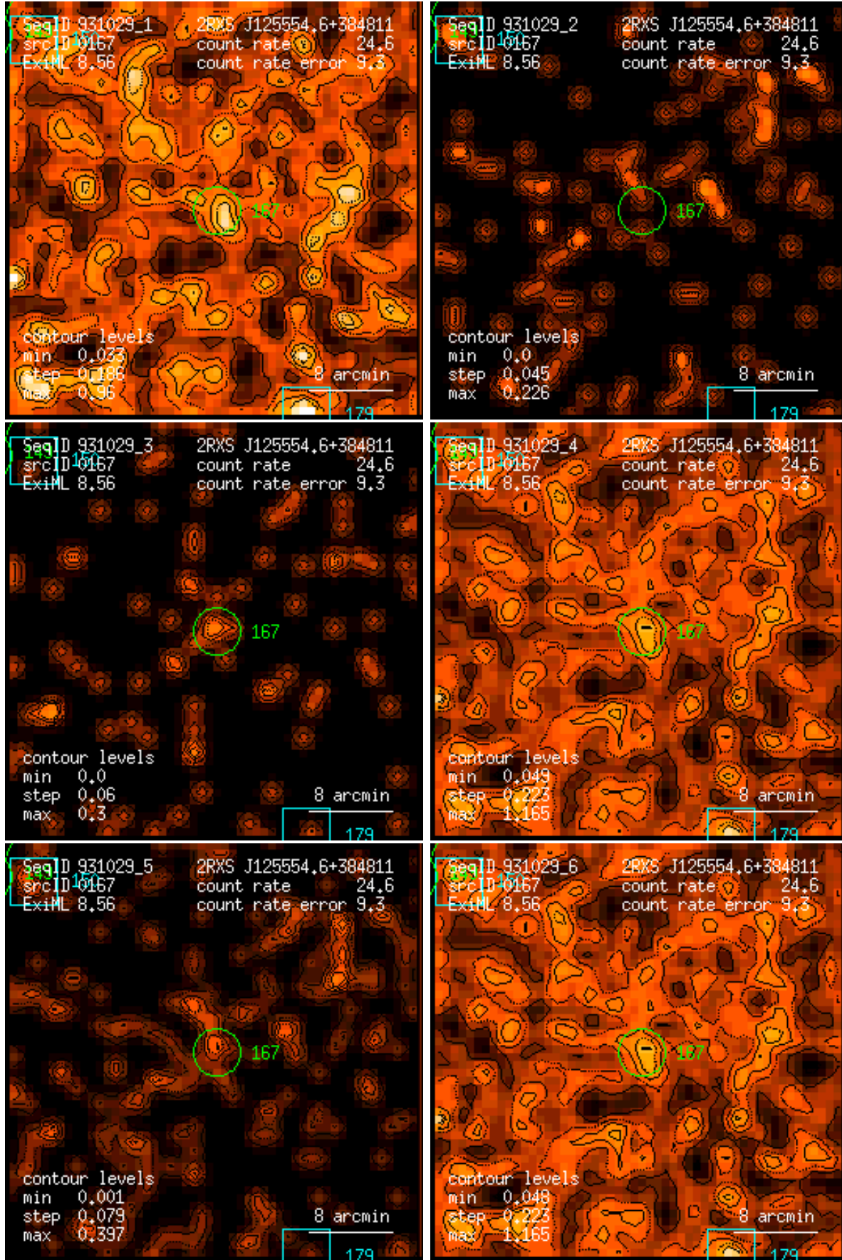
Figure 167: RASS 931029: detection 0167: band rate images, Gaussian filter: (1) PSPC channels 11 – 41, (2) 52 – 90, (3) 91 – 201, (4) 11 – 235, (5) 52 – 201, (6) 11 – 201. Broad band rates in counts/ks. Band rate contour levels in counts/ks/arcmin 2 .
