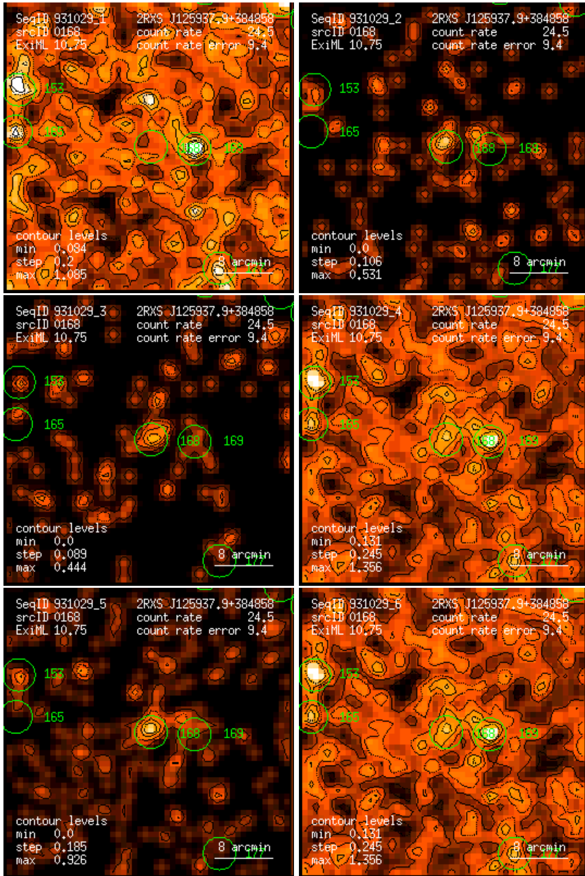
Figure 168: RASS 931029: detection 0168: band rate images, Gaussian filter: (1) PSPC channels 11 – 41, (2) 52 – 90, (3) 91 – 201, (4) 11 – 235, (5) 52 – 201, (6) 11 – 201. Broad band rates in counts/ks. Band rate contour levels in counts/ks/arcmin 2 .
