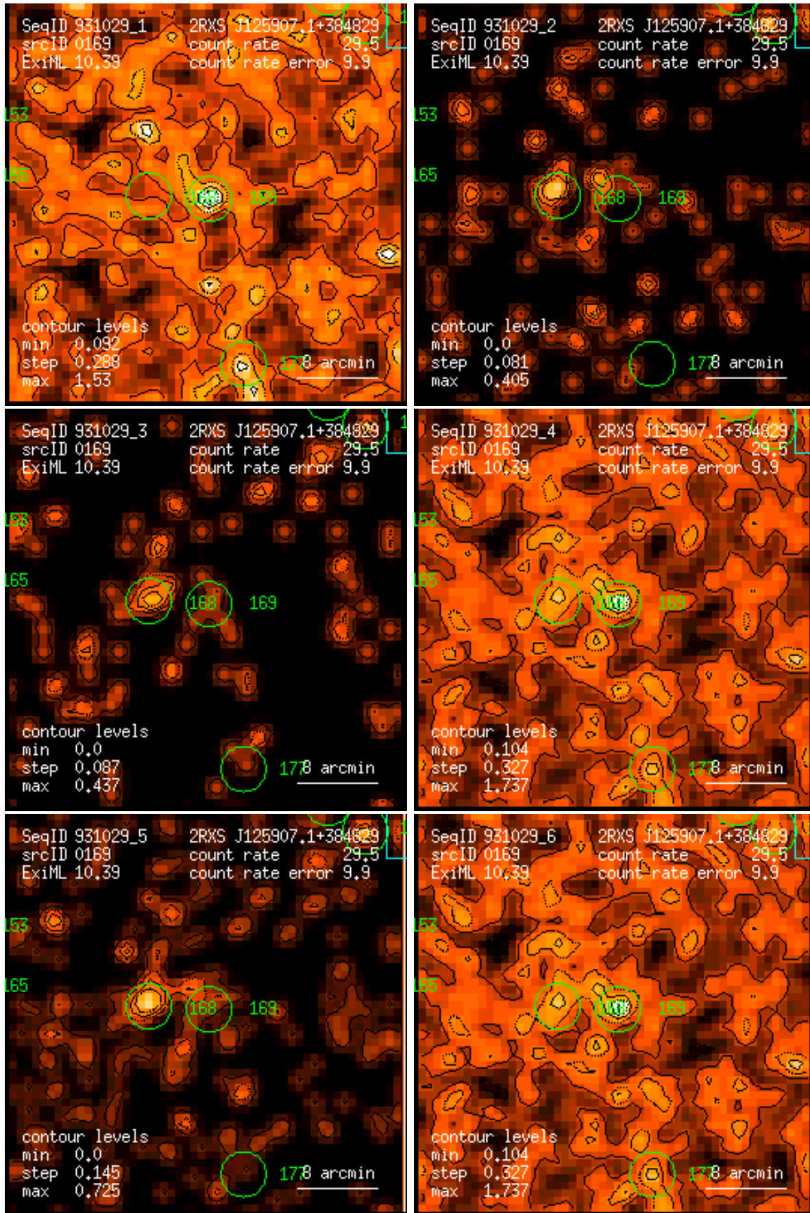
Figure 169: RASS 931029: detection 0169: band rate images, Gaussian filter: (1) PSPC channels 11 – 41, (2) 52 – 90, (3) 91 – 201, (4) 11 – 235, (5) 52 – 201, (6) 11 – 201. Broad band rates in counts/ks. Band rate contour levels in counts/ks/arcmin 2 .
