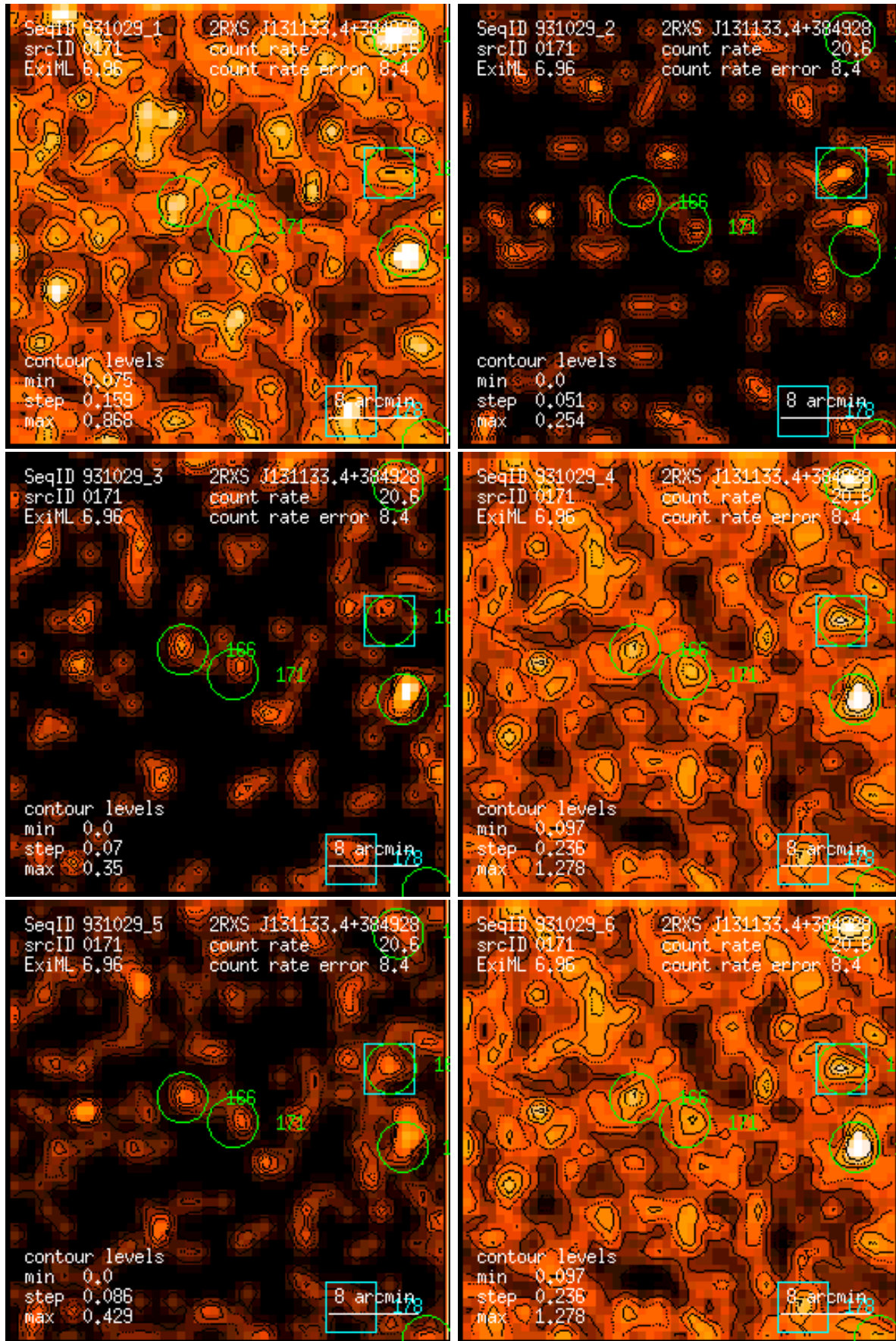
Figure 171: RASS 931029: detection 0171: band rate images, Gaussian filter: (1) PSPC channels 11 – 41, (2) 52 – 90, (3) 91 – 201, (4) 11 – 235, (5) 52 – 201, (6) 11 – 201. Broad band rates in counts/ks. Band rate contour levels in counts/ks/arcmin 2 .
