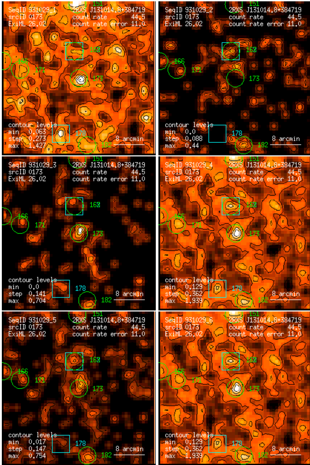
Figure 173: RASS 931029: detection 0173: band rate images, Gaussian filter: (1) PSPC channels 11 – 41, (2) 52 – 90, (3) 91 – 201, (4) 11 – 235, (5) 52 – 201, (6) 11 – 201. Broad band rates in counts/ks. Band rate contour levels in counts/ks/arcmin 2 .
