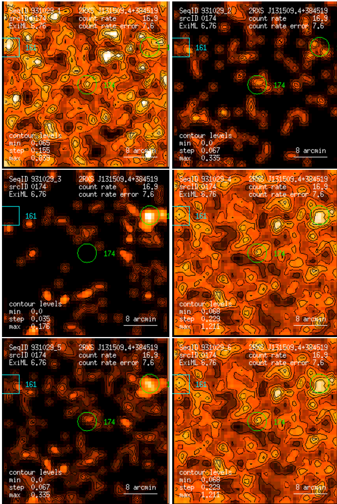
Figure 174: RASS 931029: detection 0174: band rate images, Gaussian filter: (1) PSPC channels 11 – 41, (2) 52 – 90, (3) 91 – 201, (4) 11 – 235, (5) 52 – 201, (6) 11 – 201. Broad band rates in counts/ks. Band rate contour levels in counts/ks/arcmin 2 .
