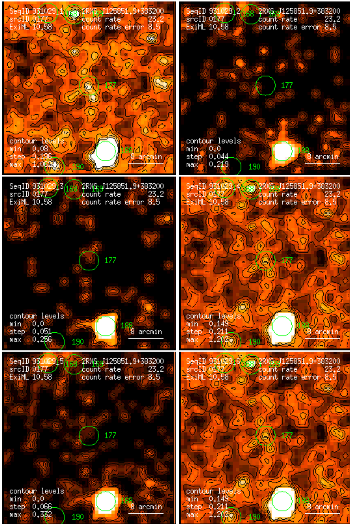
Figure 177: RASS 931029: detection 0177: band rate images, Gaussian filter: (1) PSPC channels 11 – 41, (2) 52 – 90, (3) 91 – 201, (4) 11 – 235, (5) 52 – 201, (6) 11 – 201. Broad band rates in counts/ks. Band rate contour levels in counts/ks/arcmin 2 .
