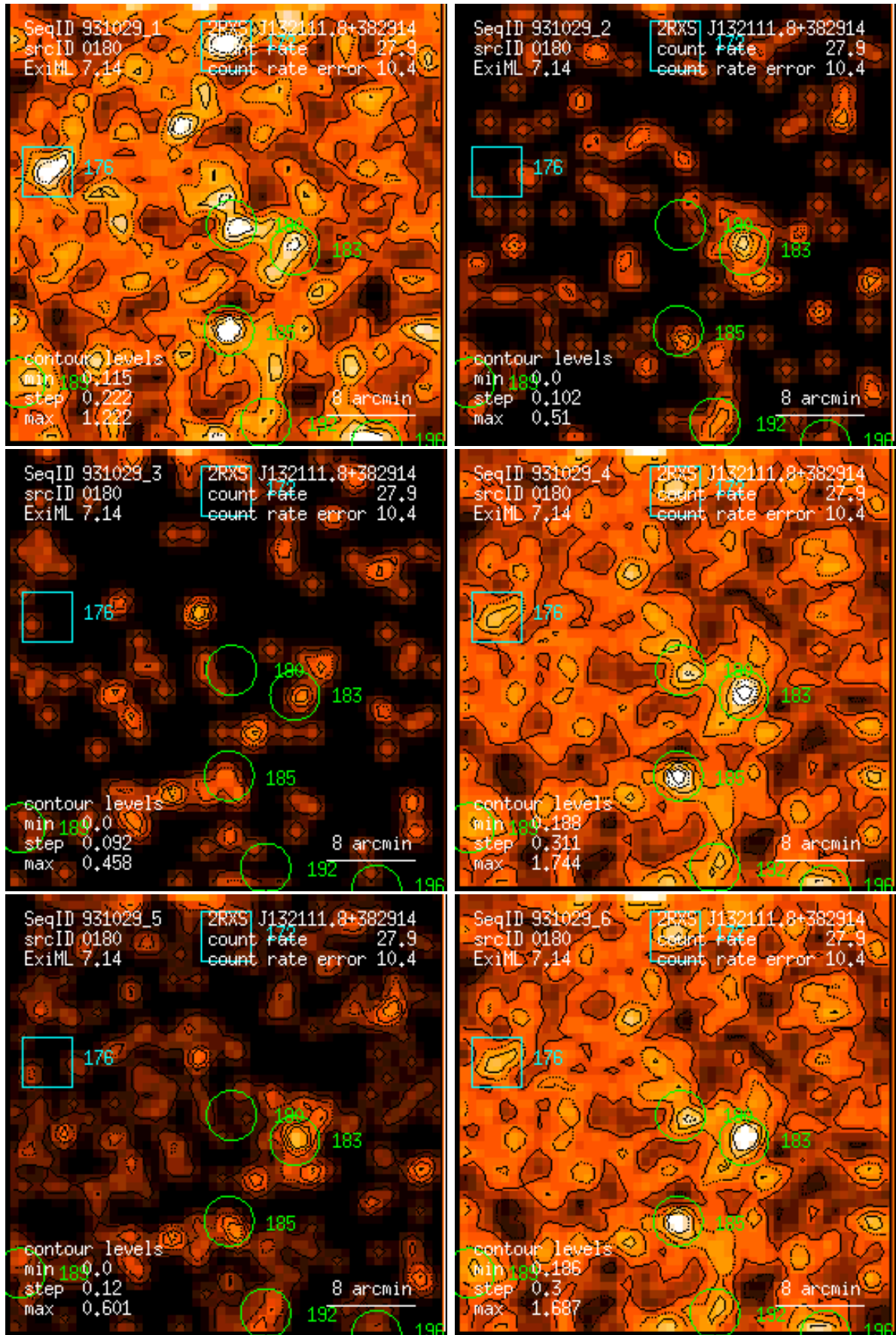
Figure 180: RASS 931029: detection 0180: band rate images, Gaussian filter: (1) PSPC channels 11 – 41, (2) 52 – 90, (3) 91 – 201, (4) 11 – 235, (5) 52 – 201, (6) 11 – 201. Broad band rates in counts/ks. Band rate contour levels in counts/ks/arcmin 2 .
