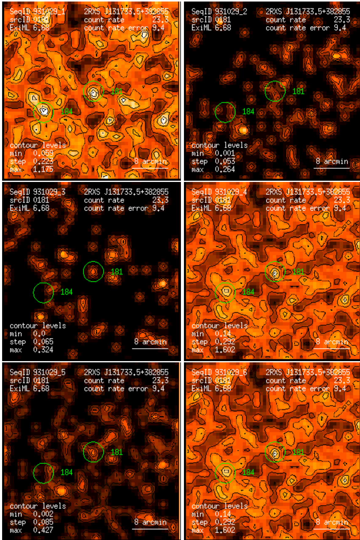
Figure 181: RASS 931029: detection 0181: band rate images, Gaussian filter: (1) PSPC channels 11 – 41, (2) 52 – 90, (3) 91 – 201, (4) 11 – 235, (5) 52 – 201, (6) 11 – 201. Broad band rates in counts/ks. Band rate contour levels in counts/ks/arcmin 2 .
