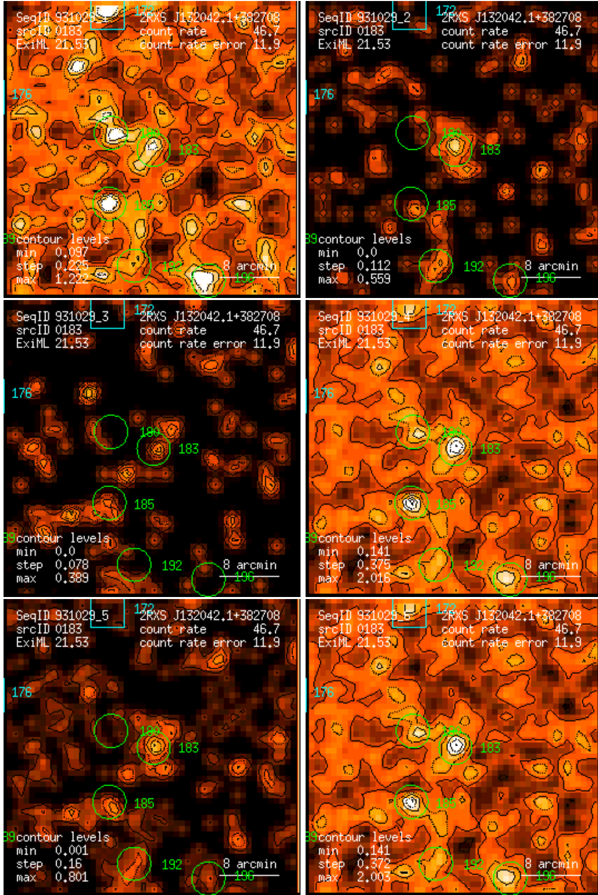
Figure 183: RASS 931029: detection 0183: band rate images, Gaussian filter: (1) PSPC channels 11 – 41, (2) 52 – 90, (3) 91 – 201, (4) 11 – 235, (5) 52 – 201, (6) 11 – 201. Broad band rates in counts/ks. Band rate contour levels in counts/ks/arcmin 2 .
