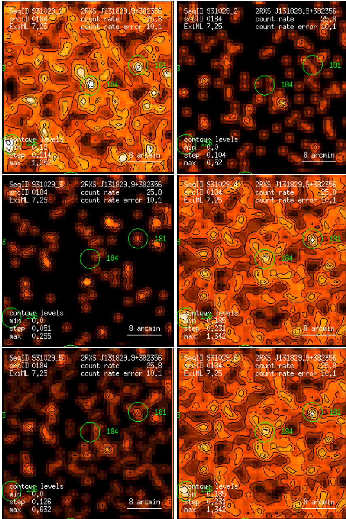
Figure 184: RASS 931029: detection 0184: band rate images, Gaussian filter: (1) PSPC channels 11 – 41, (2) 52 – 90, (3) 91 – 201, (4) 11 – 235, (5) 52 – 201, (6) 11 – 201. Broad band rates in counts/ks. Band rate contour levels in counts/ks/arcmin 2 .
