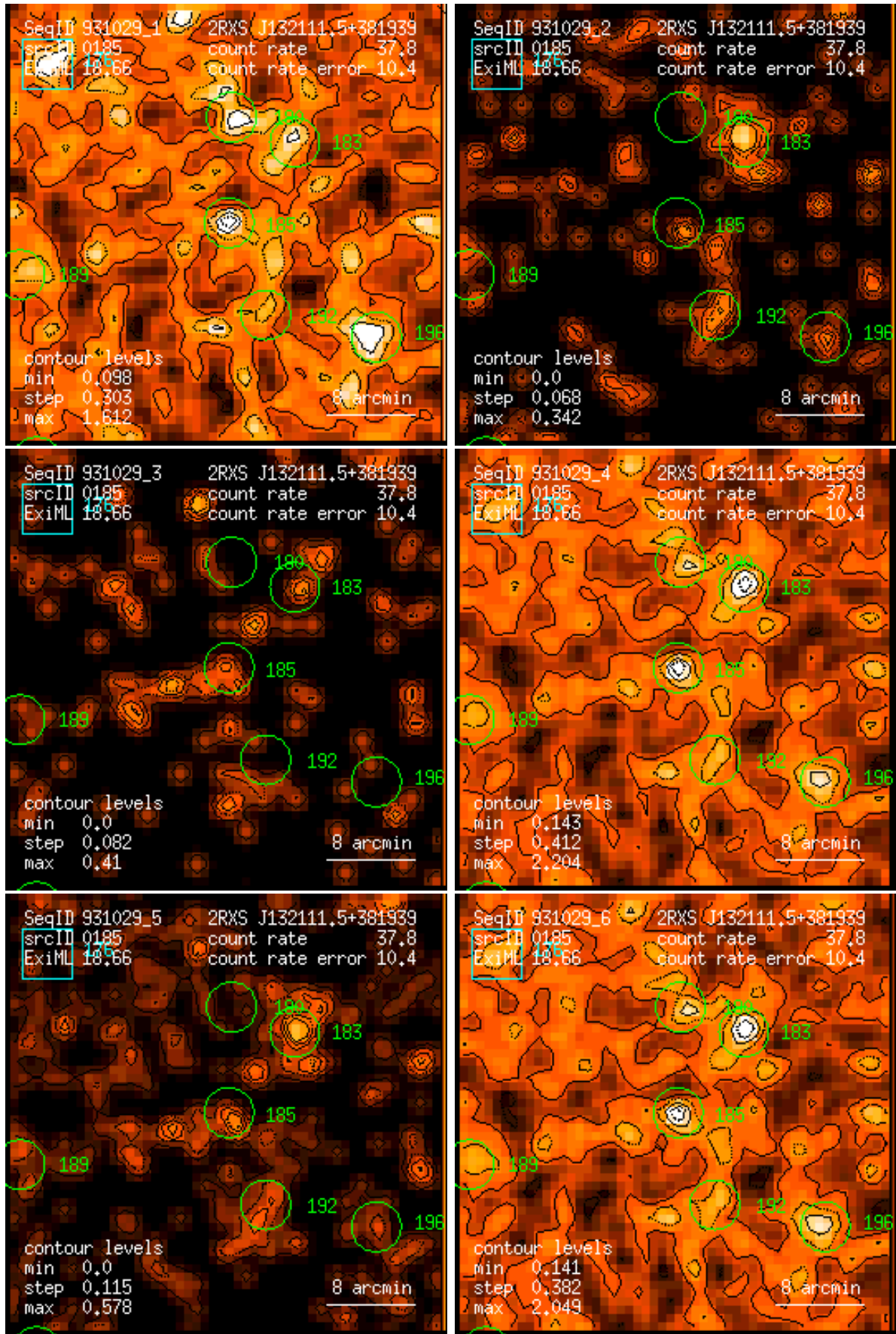
Figure 185: RASS 931029: detection 0185: band rate images, Gaussian filter: (1) PSPC channels 11 – 41, (2) 52 – 90, (3) 91 – 201, (4) 11 – 235, (5) 52 – 201, (6) 11 – 201. Broad band rates in counts/ks. Band rate contour levels in counts/ks/arcmin 2 .
