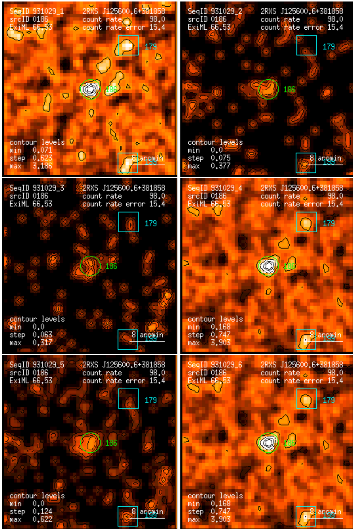
Figure 186: RASS 931029: detection 0186: band rate images, Gaussian filter: (1) PSPC channels 11 – 41, (2) 52 – 90, (3) 91 – 201, (4) 11 – 235, (5) 52 – 201, (6) 11 – 201. Broad band rates in counts/ks. Band rate contour levels in counts/ks/arcmin 2 .
