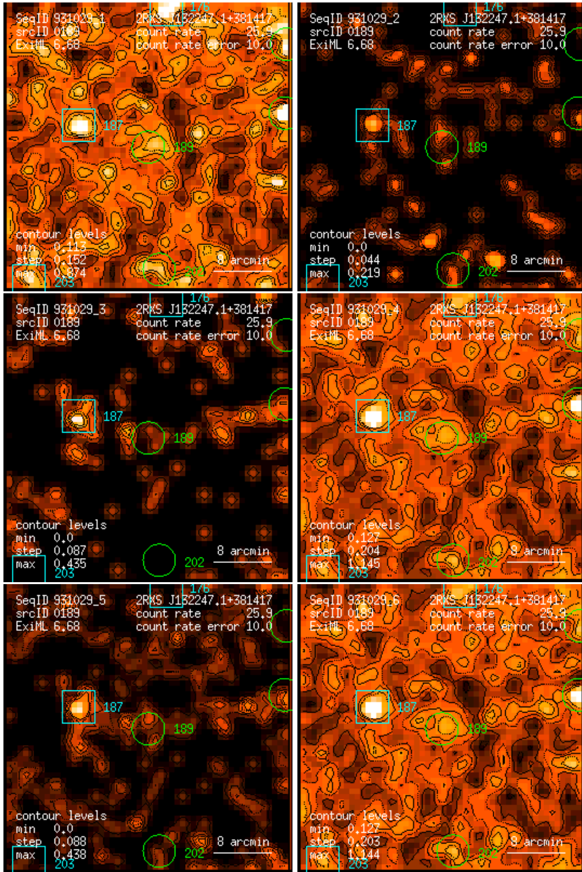
Figure 189: RASS 931029: detection 0189: band rate images, Gaussian filter: (1) PSPC channels 11 – 41, (2) 52 – 90, (3) 91 – 201, (4) 11 – 235, (5) 52 – 201, (6) 11 – 201. Broad band rates in counts/ks. Band rate contour levels in counts/ks/arcmin 2 .
