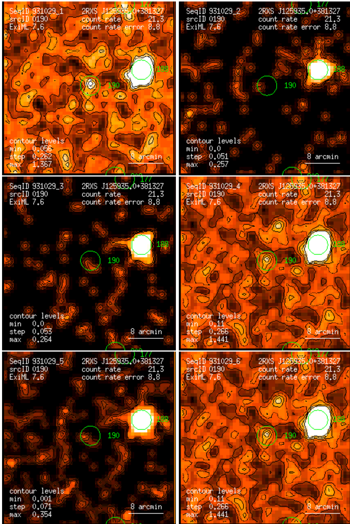
Figure 190: RASS 931029: detection 0190: band rate images, Gaussian filter: (1) PSPC channels 11 – 41, (2) 52 – 90, (3) 91 – 201, (4) 11 – 235, (5) 52 – 201, (6) 11 – 201. Broad band rates in counts/ks. Band rate contour levels in counts/ks/arcmin 2 .
