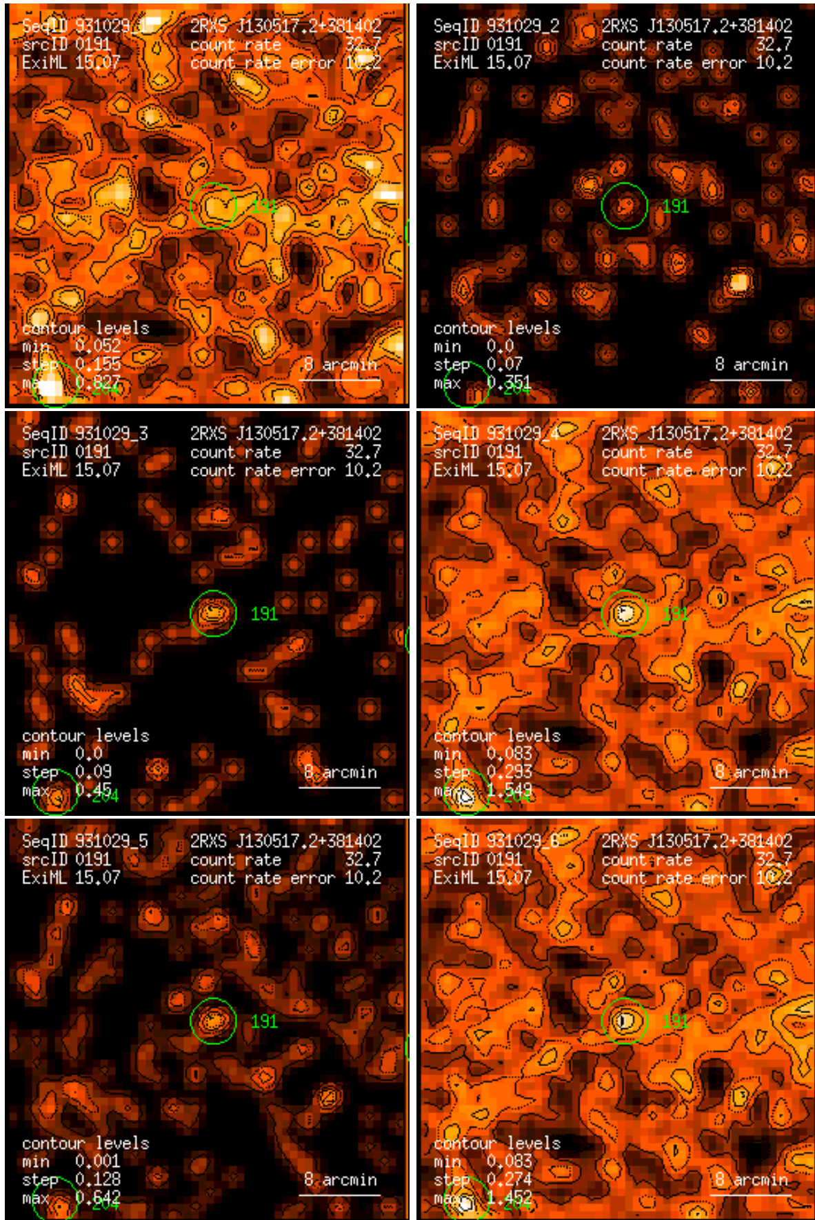
Figure 191: RASS 931029: detection 0191: band rate images, Gaussian filter: (1) PSPC channels 11 – 41, (2) 52 – 90, (3) 91 – 201, (4) 11 – 235, (5) 52 – 201, (6) 11 – 201. Broad band rates in counts/ks. Band rate contour levels in counts/ks/arcmin 2 .
