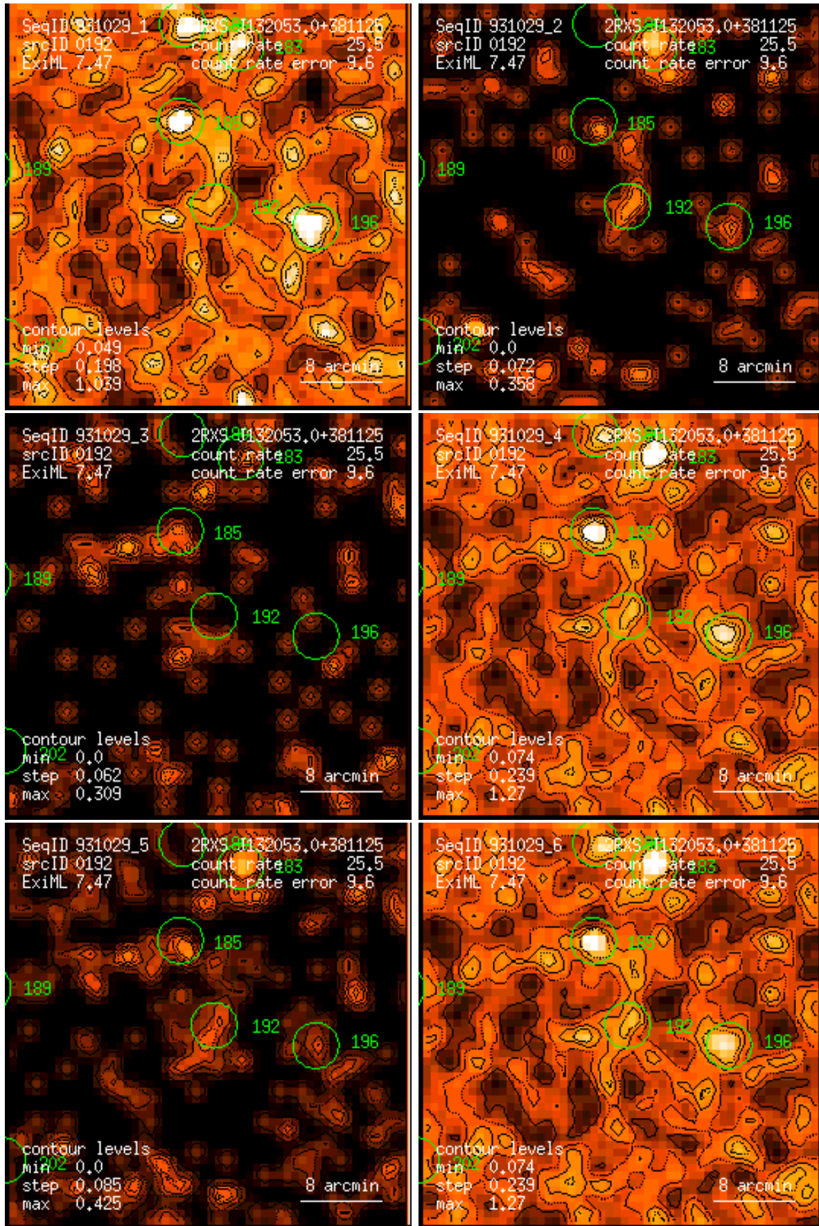
Figure 192: RASS 931029: detection 0192: band rate images, Gaussian filter: (1) PSPC channels 11 – 41, (2) 52 – 90, (3) 91 – 201, (4) 11 – 235, (5) 52 – 201, (6) 11 – 201. Broad band rates in counts/ks. Band rate contour levels in counts/ks/arcmin 2 .
