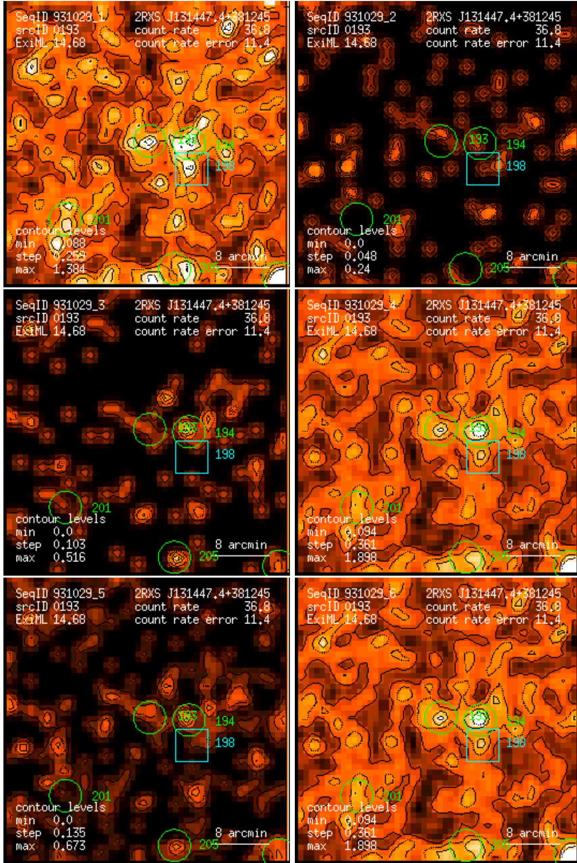
Figure 193: RASS 931029: detection 0193: band rate images, Gaussian filter: (1) PSPC channels 11 – 41, (2) 52 – 90, (3) 91 – 201, (4) 11 – 235, (5) 52 – 201, (6) 11 – 201. Broad band rates in counts/ks. Band rate contour levels in counts/ks/arcmin 2 .
