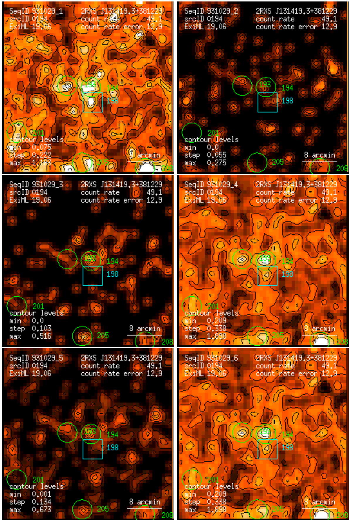
Figure 194: RASS 931029: detection 0194: band rate images, Gaussian filter: (1) PSPC channels 11 – 41, (2) 52 – 90, (3) 91 – 201, (4) 11 – 235, (5) 52 – 201, (6) 11 – 201. Broad band rates in counts/ks. Band rate contour levels in counts/ks/arcmin 2 .
