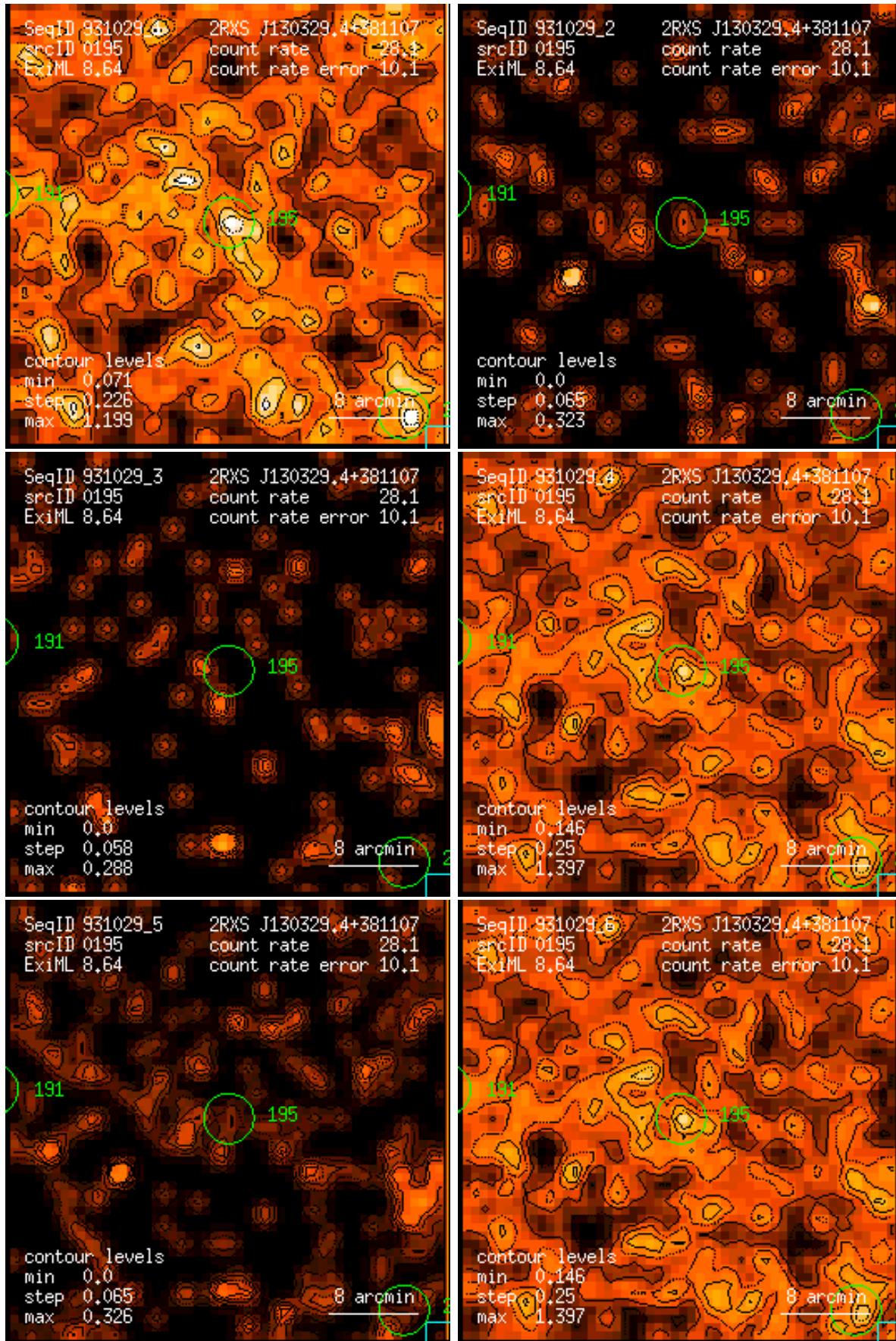
Figure 195: RASS 931029: detection 0195: band rate images, Gaussian filter: (1) PSPC channels 11 – 41, (2) 52 – 90, (3) 91 – 201, (4) 11 – 235, (5) 52 – 201, (6) 11 – 201. Broad band rates in counts/ks. Band rate contour levels in counts/ks/arcmin 2 .
