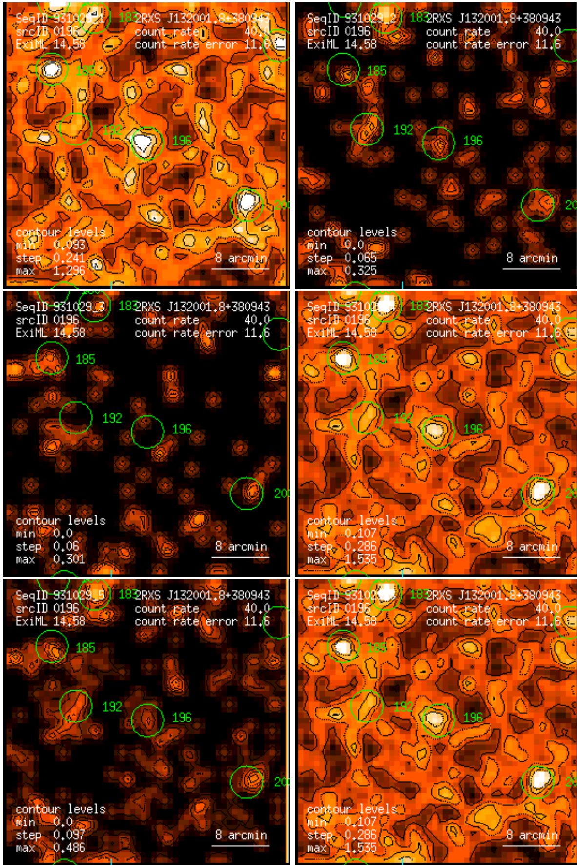
Figure 196: RASS 931029: detection 0196: band rate images, Gaussian filter: (1) PSPC channels 11 – 41, (2) 52 – 90, (3) 91 – 201, (4) 11 – 235, (5) 52 – 201, (6) 11 – 201. Broad band rates in counts/ks. Band rate contour levels in counts/ks/arcmin 2 .
