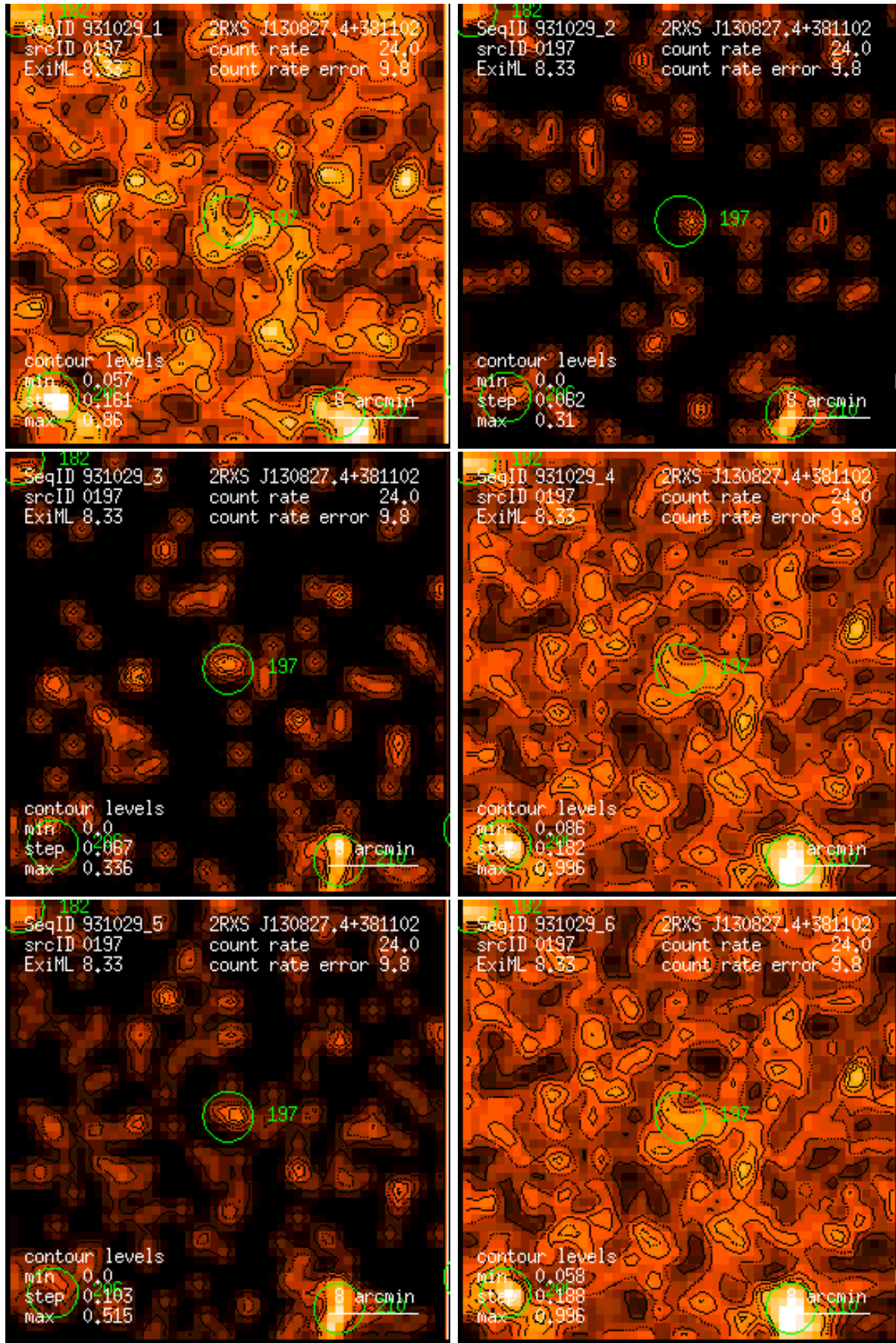
Figure 197: RASS 931029: detection 0197: band rate images, Gaussian filter: (1) PSPC channels 11 – 41, (2) 52 – 90, (3) 91 – 201, (4) 11 – 235, (5) 52 – 201, (6) 11 – 201. Broad band rates in counts/ks. Band rate contour levels in counts/ks/arcmin 2 .
