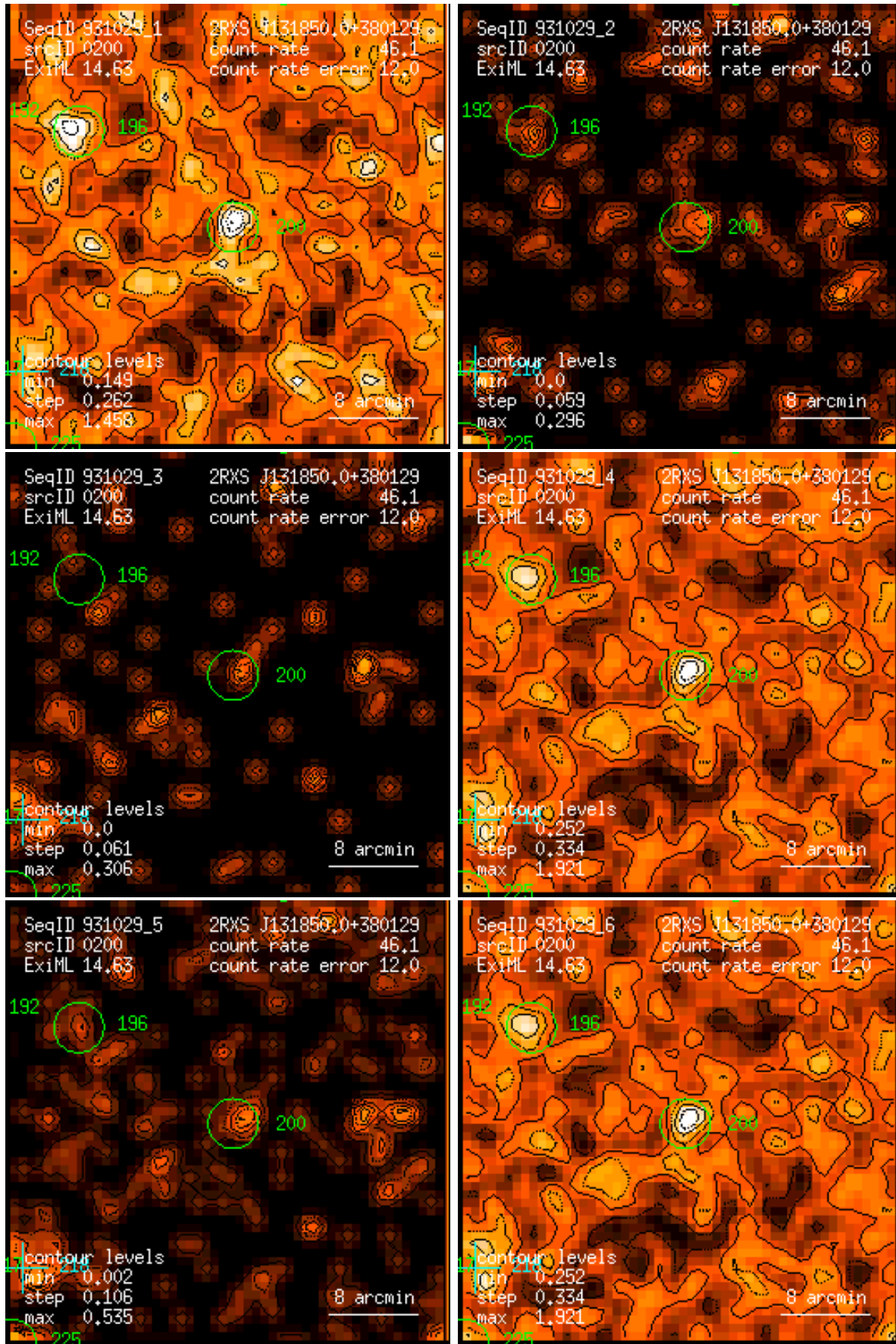
Figure 200: RASS 931029: detection 0200: band rate images, Gaussian filter: (1) PSPC channels 11 – 41, (2) 52 – 90, (3) 91 – 201, (4) 11 – 235, (5) 52 – 201, (6) 11 – 201. Broad band rates in counts/ks. Band rate contour levels in counts/ks/arcmin 2 .
