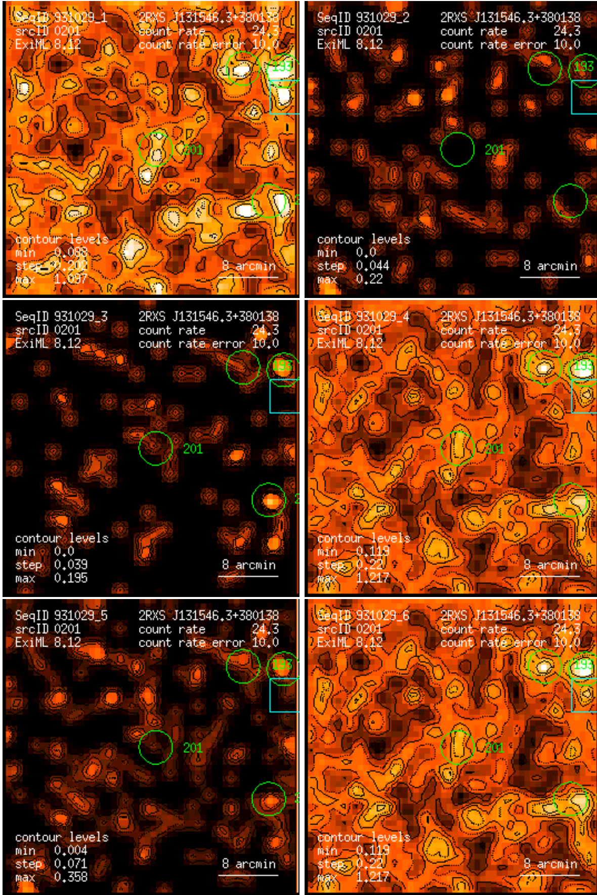
Figure 201: RASS 931029: detection 0201: band rate images, Gaussian filter: (1) PSPC channels 11 – 41, (2) 52 – 90, (3) 91 – 201, (4) 11 – 235, (5) 52 – 201, (6) 11 – 201. Broad band rates in counts/ks. Band rate contour levels in counts/ks/arcmin 2 .
