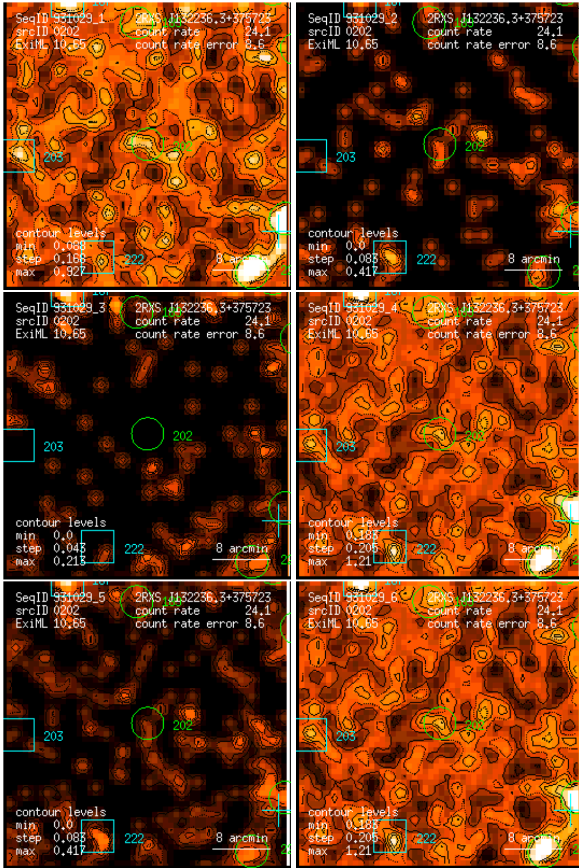
Figure 202: RASS 931029: detection 0202: band rate images, Gaussian filter: (1) PSPC channels 11 – 41, (2) 52 – 90, (3) 91 – 201, (4) 11 – 235, (5) 52 – 201, (6) 11 – 201. Broad band rates in counts/ks. Band rate contour levels in counts/ks/arcmin 2 .
