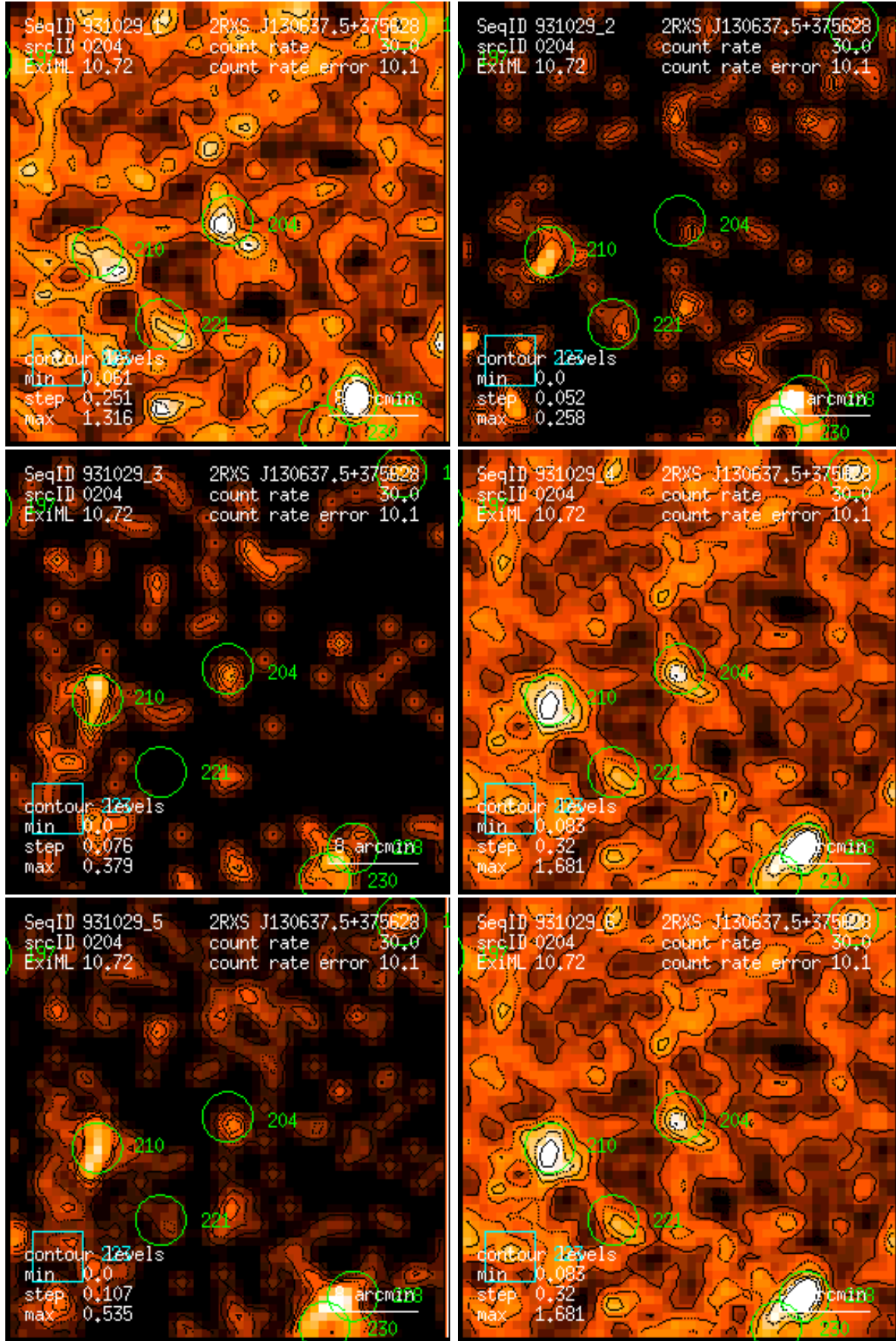
Figure 204: RASS 931029: detection 0204: band rate images, Gaussian filter: (1) PSPC channels 11 – 41, (2) 52 – 90, (3) 91 – 201, (4) 11 – 235, (5) 52 – 201, (6) 11 – 201. Broad band rates in counts/ks. Band rate contour levels in counts/ks/arcmin 2 .
