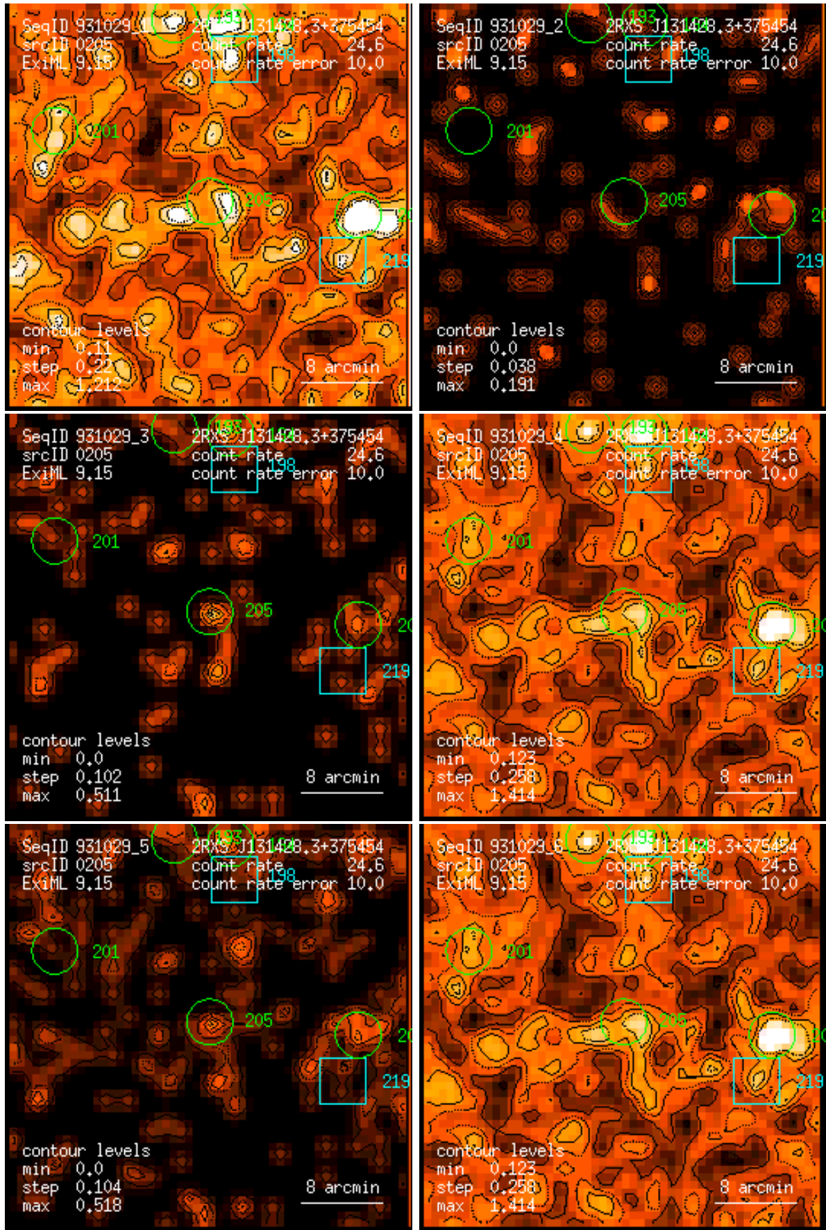
Figure 205: RASS 931029: detection 0205: band rate images, Gaussian filter: (1) PSPC channels 11 – 41, (2) 52 – 90, (3) 91 – 201, (4) 11 – 235, (5) 52 – 201, (6) 11 – 201. Broad band rates in counts/ks. Band rate contour levels in counts/ks/arcmin 2 .
