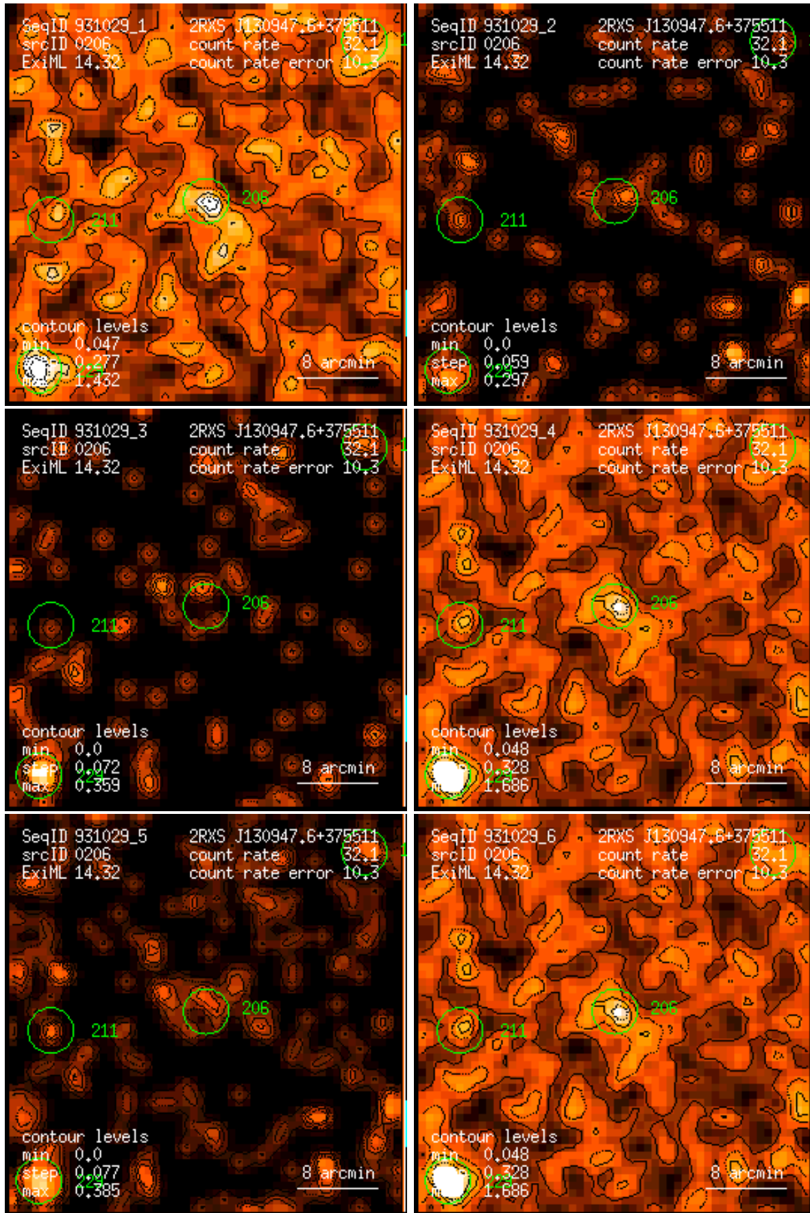
Figure 206: RASS 931029: detection 0206: band rate images, Gaussian filter: (1) PSPC channels 11 – 41, (2) 52 – 90, (3) 91 – 201, (4) 11 – 235, (5) 52 – 201, (6) 11 – 201. Broad band rates in counts/ks. Band rate contour levels in counts/ks/arcmin 2 .
